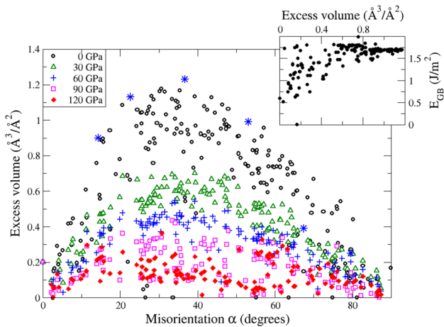
Fig. 5 Evolution of GB excess volumes with pressure. Excess volume is reported versus the misorientation for ambient pressure (open circles), and pressures equal to 30 GPa (open triangles), 60 GPa (crosses), 90 GPa (open squares), and 120 GPa (filled diamonds). The blue stars are the data at ambient pressure from Yokoi and Yoshiya (2017). The inset graph shows the relationship between formation energies and excess volumes at 0 GPa, for all GB studied
