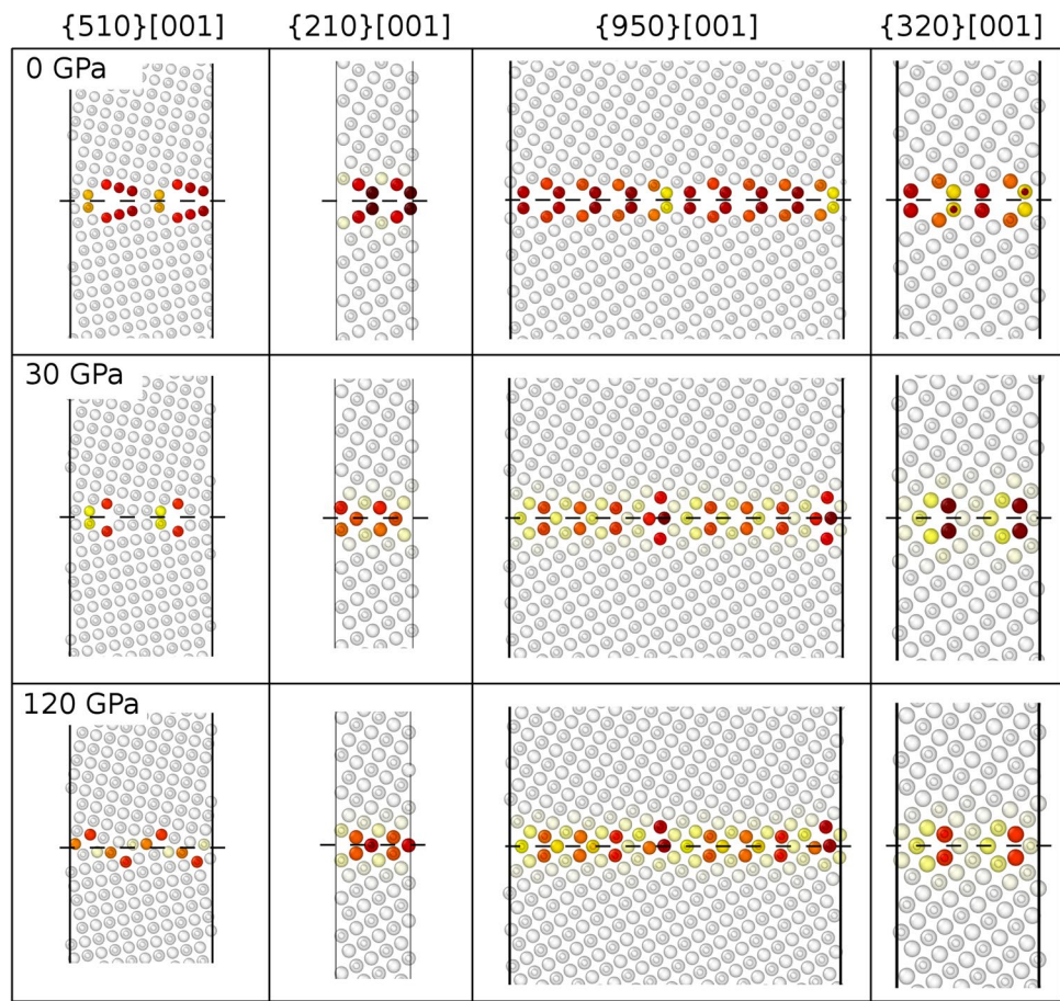
Fig. 3 Evolution with pressure of the optimal atomic configuration of some high-angle GBs (same colour convention, as shown in Fig. 2). The grain boundaries are: \{510\} [001] ( \alpha=22.6^\circ ); \{210\} [001] ( \alpha=53.1^\circ ); \{950\} [001] ( \alpha=58.1^\circ ); \{320\} [001] ( \alpha=67.4^\circ )
