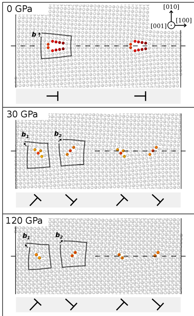
Fig. 2 Evolution with pressure of the optimal atomic configuration of a low-angle ( \alpha=5.2^\circ ) tilt GB. Atoms in near-perfect environment are displayed in light grey, those in defects appear in colour, according to their central symmetry parameter (Kelchner et al. 1998). The [001] direction is normal to the figure, and the GB plane, indicated by the horizontal dashed line, is normal to the [010] direction. Burgers circuits are drawn around some dislocations. At 0 GPa, the closing Burgers vector is \mathbf{b} = [010] ; at 30 GPa and above, it decomposes into two dislocations of Burgers vectors \mathbf{b}_1 = \frac{1}{2}[-110] and \mathbf{b}_2 = \frac{1}{2}[110] . Visualization performed with OVITO (Stukowski 2010)
