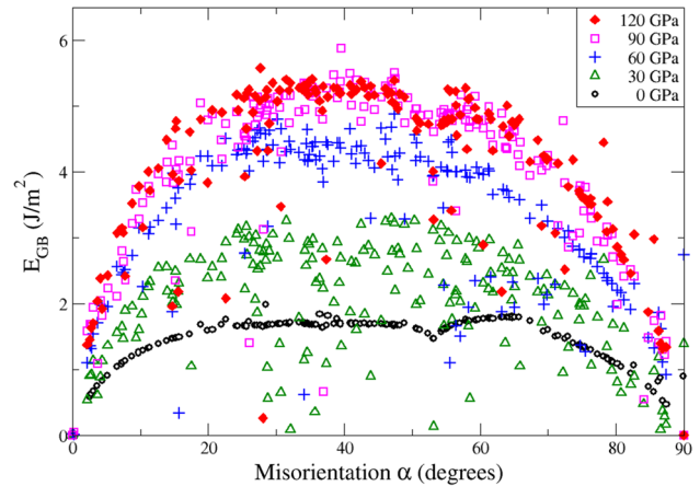
Fig. 6 Evolution with pressure of the enthalpy of formation of grain boundaries as a function of the tilt angle at 0 GPa (open circles, same as Fig. 1), 30 GPa (open triangles), 60 GPa (crosses), 90 GPa (open squares), and 120 GPa (filled diamonds)
