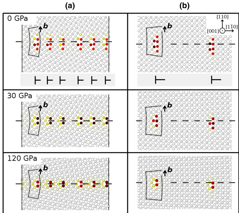
Fig. 4 Evolution with pressure of the atomic configuration of near-right angle STGBs. The misorientations between the two crystals are: a \alpha = 70^\circ ; b \alpha = 84.8^\circ . Those GBs decompose into an array of \frac{1}{2}[110] (1–10) edge dislocations, as schematized by the \perp signs (same colour conventions, as shown in Fig. 2). The crystal directions are given for GBs in column b , where the GB plane is almost normal to the [110] direction. Note that since each crystal was rotated by an angle close to 45^\circ , the crystal directions are different from Fig. 2
