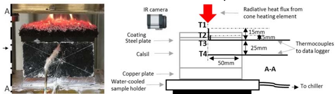
Fig. 1. Experimental set-up.
