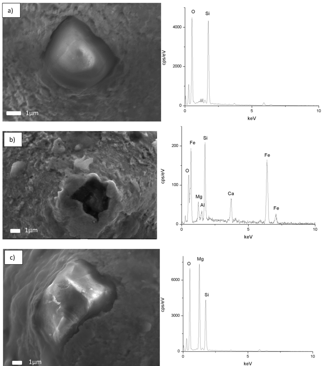
Fig. 2. SEM images and EDS spectra of typical inclusions found on fracture surfaces. a) SiO 2 ; b) SiO 2 -CaO; c) SiO 2 -MgO.
