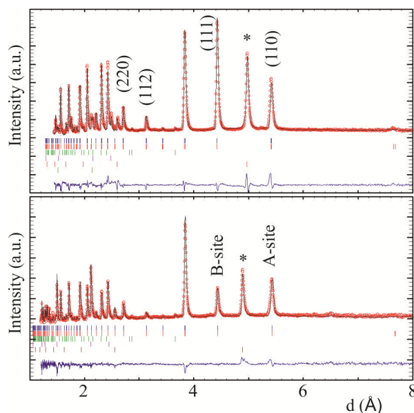
FIGURE 1. Rietveld fits of NPD patterns collected at 1.5 K for CaMnCoReO 6 (top) and CaMnNiReO 6 (bottom). Bragg markers from top to bottom are the nuclear and magnetic structures of the DDPv phase, ReO 2 and the nuclear and magnetic structures of M 0.67 Mn 0.33 O. The main magnetic peaks are indexed on the top panel and the perovskite-superstructure peaks evidencing the A- and B-site cation orders are identified at the bottom. The main magnetic peak of M 0.67 Mn 0.33 O is marked *.
