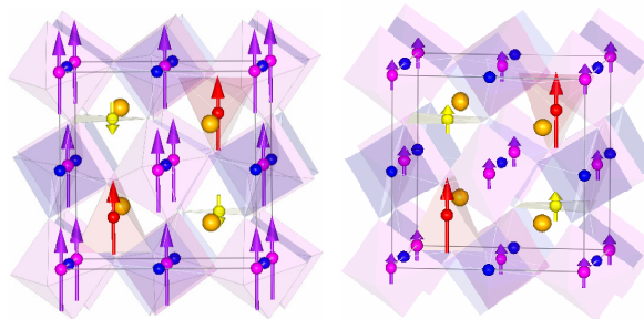
FIGURE 3. Crystal and magnetic structures of CaMnCoReO 6 (left) and CaMnNiReO 6 (right) with the z-axis vertical. Orange, red, yellow, purple and blue spheres represent Ca, A', A'', B and Re sites respectively. Polyhedra show the tetrahedral, square planar and octahedral coordination of A', A'' and B sites, and arrows show the spin directions scaled to the refined magnitudes of the ordered moments.
