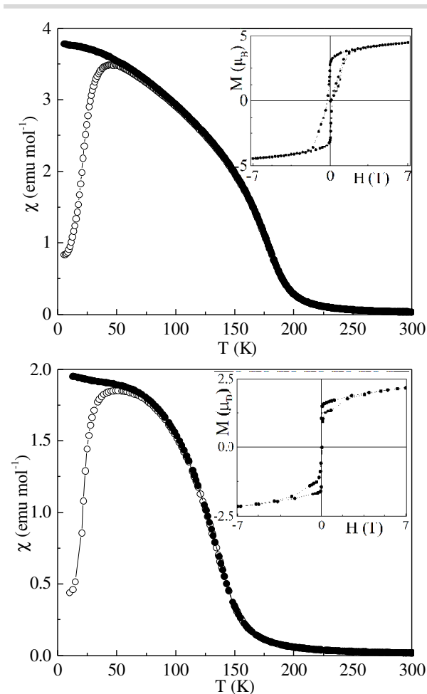
FIGURE 2. Magnetic susceptibilities of CaMnCoReO 6 (top) and CaMnNiReO 6 (bottom) with insets showing magnetization-field loops at 7 and 2 K respectively.
