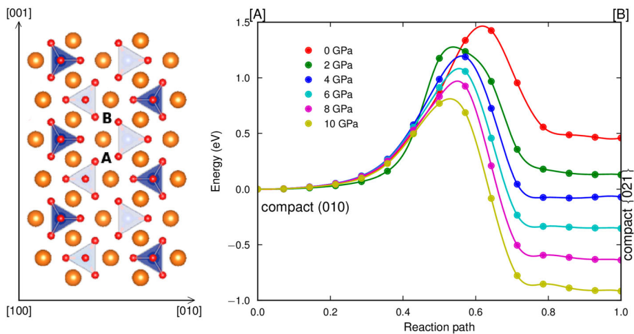
Figure 6. MEP associated with the transition from a compact (010) core to a compact (021) configuration, i.e between [A] and [B] sites in (010). The energies are given for a dislocation line of length b.
