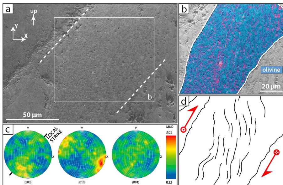
Figure 12. Vertical section revealing a relationship between CPO and shape preferred orientation in microcrystalline olivine. (a) polished surface showing microcrystalline grains of the fault gouge, located in Figure 4e; (b) phase map indicating olivine indexation in blue; (c) electron backscatter diffraction pole figures (in plane) showing olivine CPO consistent with results presented in Figure 6; (d) simple sketch highlighting S-C fabric and related sense of shear. The horizontal sense of shear is also indicated. In addition, olivine grains are elongated along their [100] axis. Pink color: absence of indexed olivine. Upper stereographic projection. MUD = multiples of uniform distribution. Analysis points number: 25422. Indexation: 56.88%. Olivine: 91.4%.
