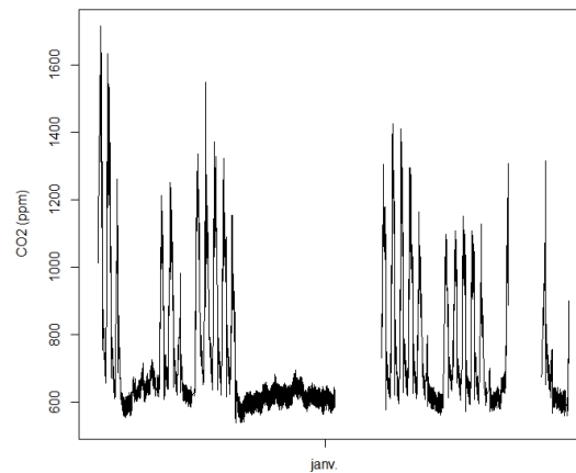
Figure 5. CO 2 concentration in the Lilliad Learning Center, from December 1, 2018 to January 25, 2019.
