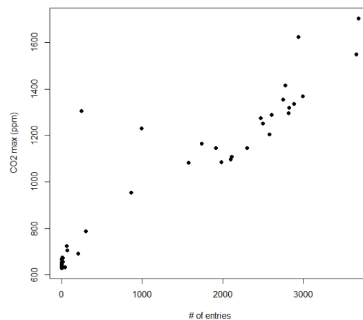
Figure 6. Correlation of the daily maximal CO 2 level with the number of entries in the Lilliad Learning Center.
