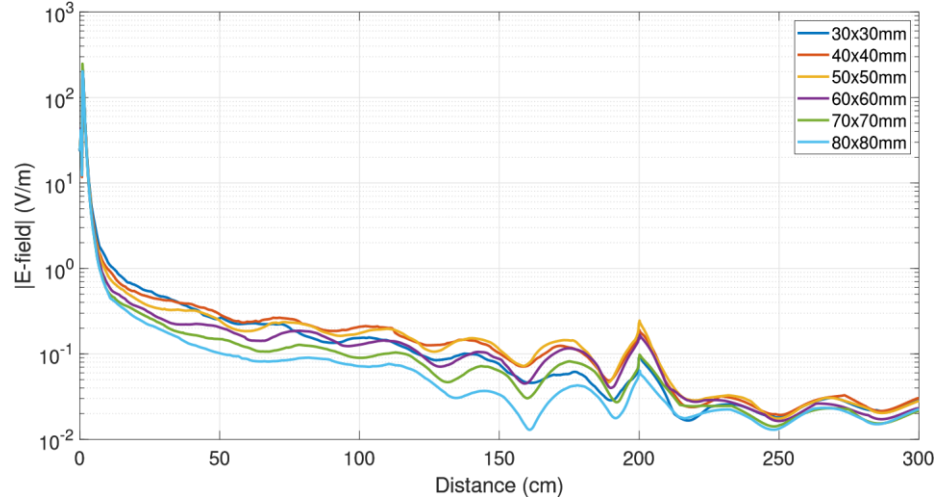
Fig.12. E-field radiated by a single electrode along the Y-axis on muscle for multiple phantom cross section at 450 MHz.
