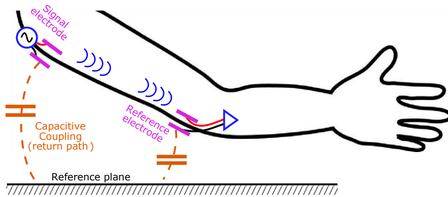
Fig.1. Common representation of Capacitive Body Coupled Communication mechanism.
