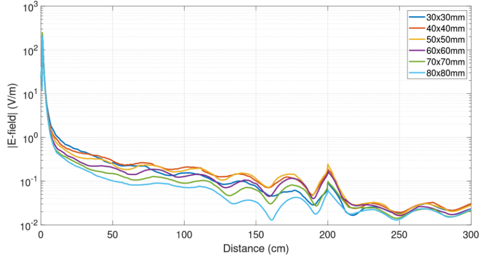
Fig.12. E-field radiated by a single electrode along the Y-axis on muscle for multiple phantom cross section at 450 MHz.
