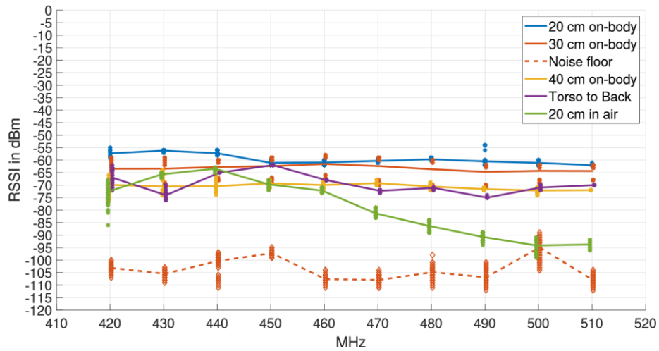
Fig.15. On-body channel loss for multiple distances.
