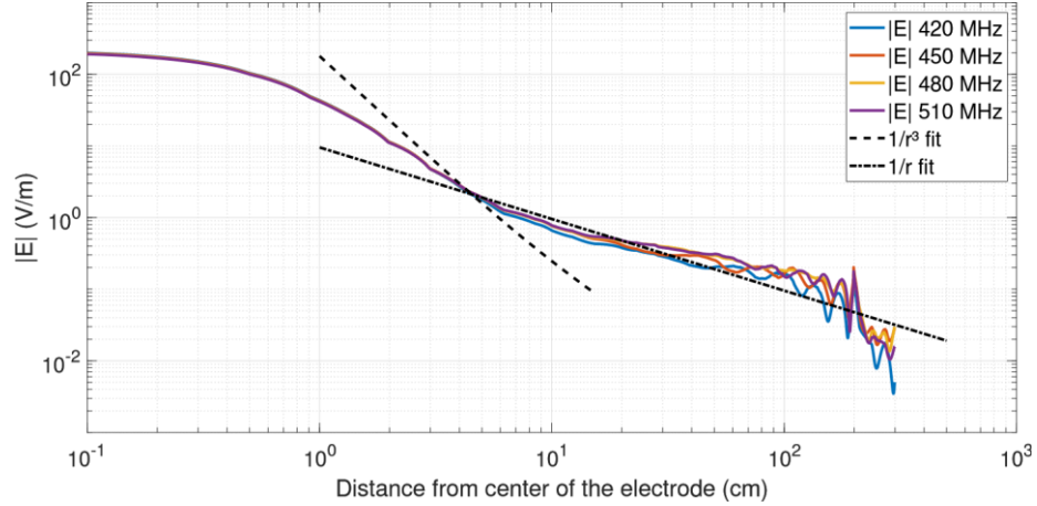
Fig.10. E-field along the Y-axis radiated by a single electrode on muscle for multiple frequencies on a 50 x 50 mm 2 phantom section.
