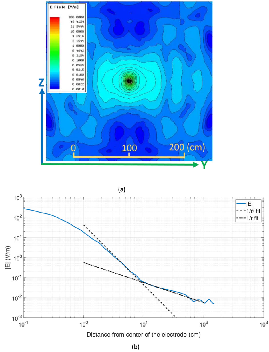
Fig.8. E-field radiated by one electrode in air at 450 MHz, (a) in the (YZ) plane, (b) along the positive Y-axis.
