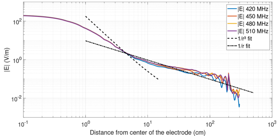
Fig.10. E-field along the Y-axis radiated by a single electrode on muscle for multiple frequencies on a 50 \times 50 \text{ mm}^2 phantom section.
