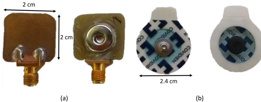
Fig.7. C-BCC electrode. (a) connector (2 x 2 cm), (b) skin pre-gelled.
