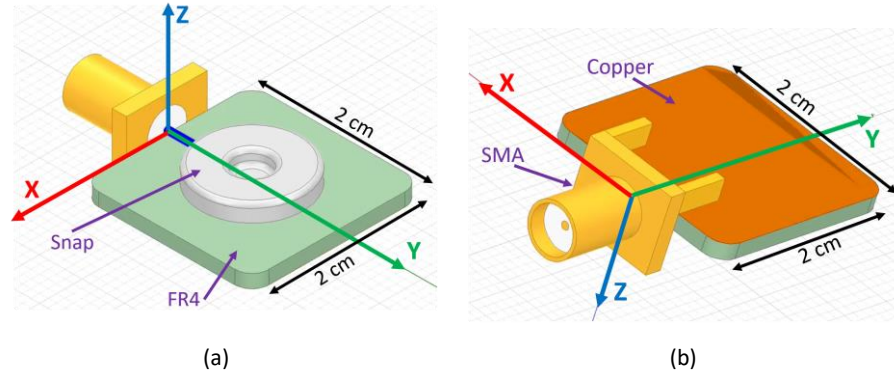
Fig.4. 3D electrode model. (a) top view, (b) bottom view.
