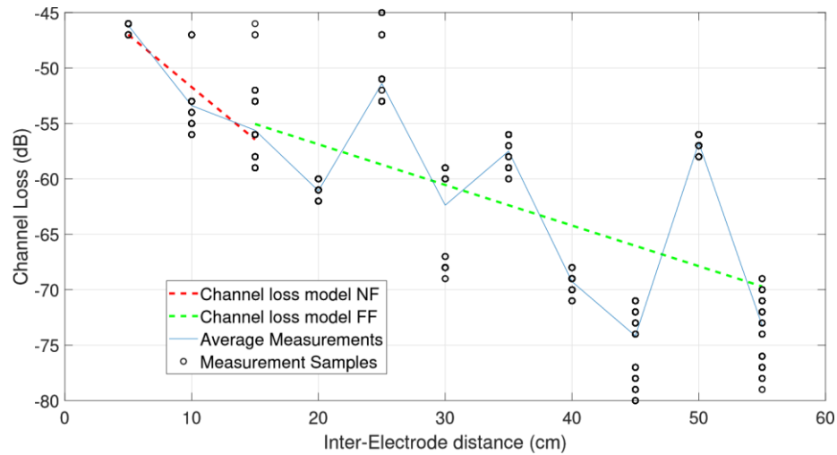
Fig.14. Channel loss measurements along the arm of a human subject at 450 MHz (black markers). The red and green lines show the two-slope channel loss model described in Eq. 3, fitted to the measurement data.
