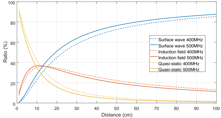
Fig.3. Contribution of each mechanism as a proportion of the total electric field for 400 MHz (dotted lines) and 500 MHz (solid lines).
