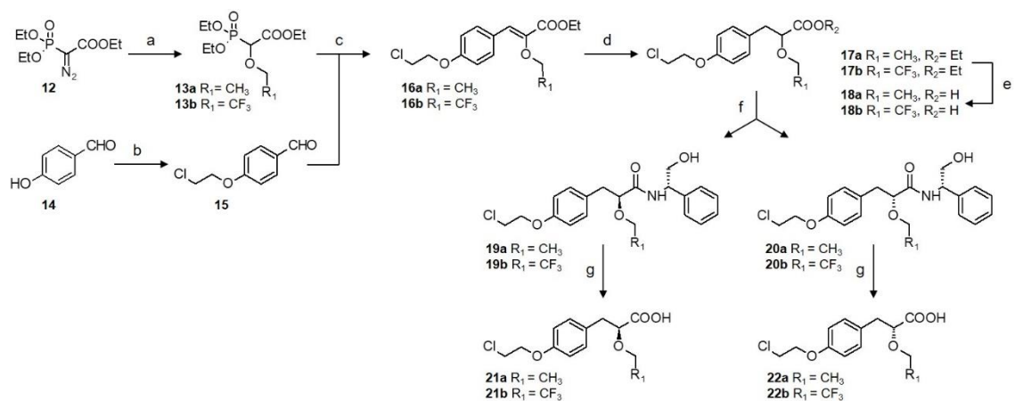
Scheme 2. Synthesis of optically pure \alpha -alkoxyphenylpropionic acids 21 , 22 . Reagents and conditions: a) ethanol or trifluoroethanol [ \text{Rh}(\text{OAc})_2 ] 2 , toluene, reflux; b) 1,2-bromo-chloroethane, \text{K}_2\text{CO}_3 , \text{CH}_3\text{CN} , reflux; c) \text{NaH} , dry THF, 0^\circ\text{C} to r.t.; d) \text{H}_2 , \text{Pd/C} , ethanol, r.t.; e) \text{LiOH} , THF/ \text{H}_2\text{O} , r.t.; f) 1-ethyl-3-(3-dimethylaminopropyl)-carbodiimide hydrochloride, triethylamine, HOBT, ( S )-(-)-2-phenylglycinol, DCM, 0^\circ\text{C} to r.t.; g) 5 M \text{H}_2\text{SO}_4 , dioxane/ \text{H}_2\text{O} , reflux.
