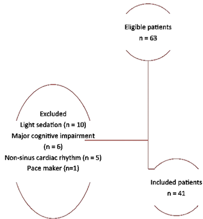
Fig 3. Study flowchart.
