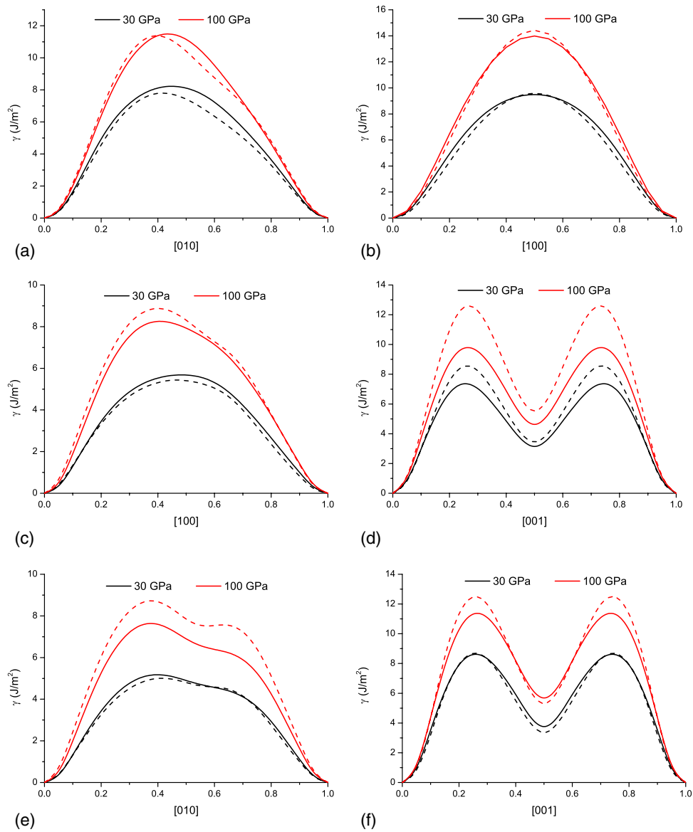
Figure 2. Comparison between pairwise potential calculations (straight line) and DFT results (dotted lines) for a selection of \gamma -lines. \gamma -lines along [0 1 0] (a) and [1 0 0] (b) in (0 0 1), along [1 0 0] (c) and along [0 0 1] (d) in (0 1 0), along [0 1 0] (e) and [0 0 1] (f) in (1 0 0). For comparison, \gamma -lines are plotted as a function of normalized shear vectors.
