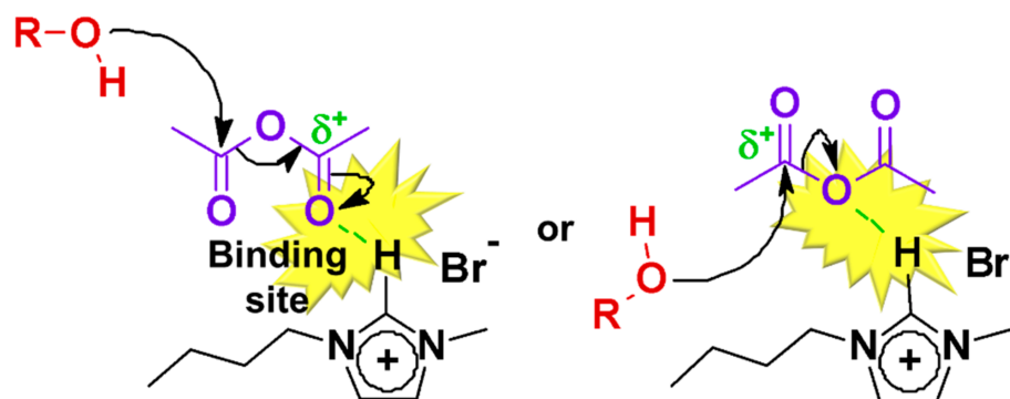
Figure 40. Possible H-bond activation with H-bond formation during O-acetylation of alcohols with acetic anhydride in 1-butyl-3-methylimidazolium bromide under sonication at 30 °C.
