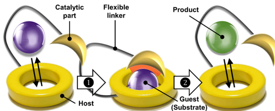
Figure 3. The general principle of “chemzymes” (1 = formation of the “chemzyme”–substrate complex and 2 = catalytic transformation).
