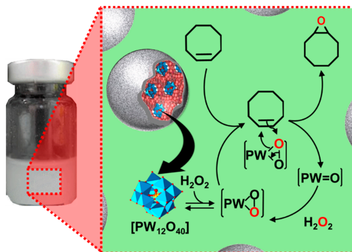
Figure 57. The mechanism of olefin epoxidation inside a colloidal solution suspension (sol) of dodecyltrimethylammonium/ \text{PW}_{12}\text{O}_{40} NPs in a continuous aqueous medium.
