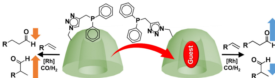
Figure 17. Cyclodextrin–phosphine with a guest-tunable conformation for biphasic, aqueous, and rhodium-catalyzed hydroformylation.
