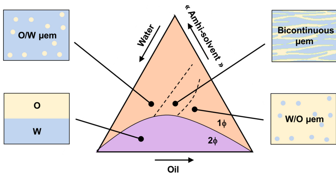
Figure 35. A schematic phase diagram of an “amphi-solvent”/water/oil ternary system and surfactant-free microemulsion types.
