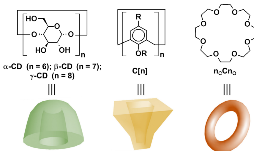
Figure 2. The structure and a schematic representation of different macrocycles ( n_C = carbon number and n_o = oxygen number). CD, cyclodextrin; C, calixarene; nCn, crown ether.
