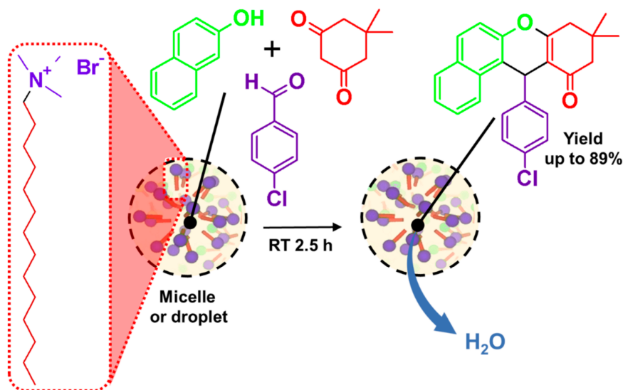
Figure 24. Synthesis of 12-(4-chlorophenyl)-9,9-dimethyl-8,9,10,12-tetrahydrobenzo[a] xanthen-11-one catalyzed by a tetradecyltrimethylammonium bromide surfactant at room temperature.
