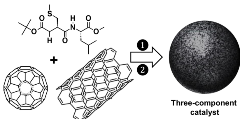
Figure 47. The self-assembly of a terminally protected hydrophobic dipeptide (Boc-L-Cys(Me)-L-Leu-OMe) with carbon-based materials (carbon nanotubes and fullerene C_{60} ) to obtain a ternary catalyst (1: formation of organogel, and 2: vacuum drying).
