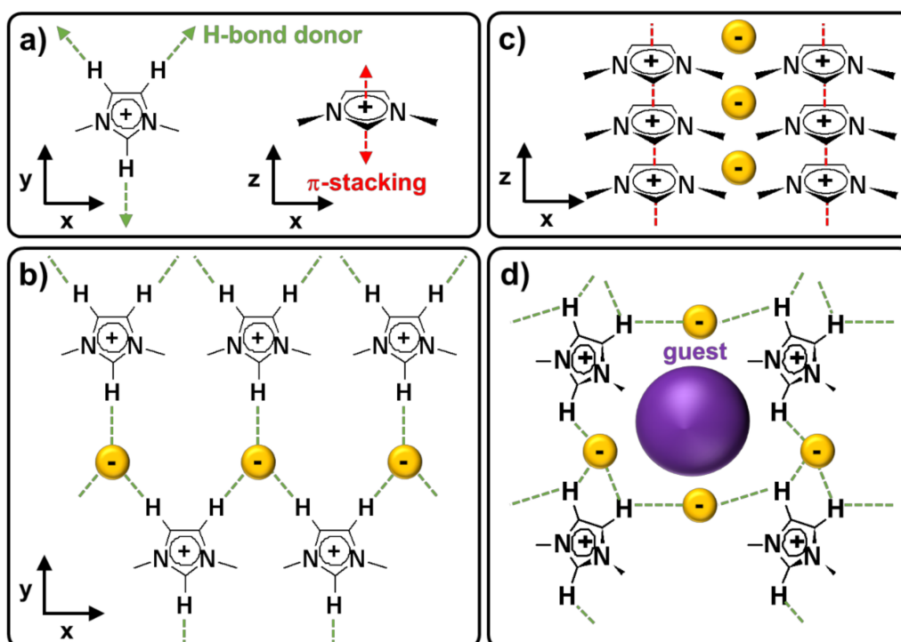
Figure 38. (a) H-bond donors (green) and \pi -stacking (red) of an imidazolium ring; (b,c) simplified two-dimensional (2-D) and three-dimensional (3-D) organization of the imidazolium salt; (d) the local assembly of the imidazolium ILs around guest molecules.
