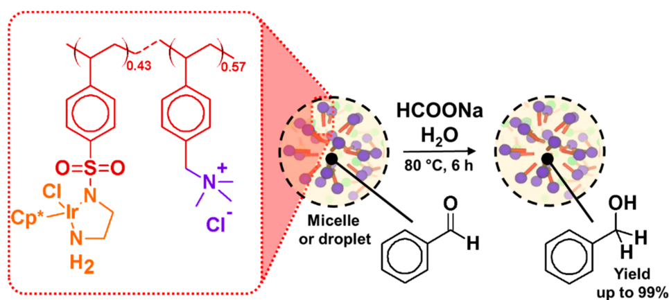
Figure 25. Catalytic hydrogenation of aldehydes using an amphiphilic polymer combined with an iridium organometallic complex.
