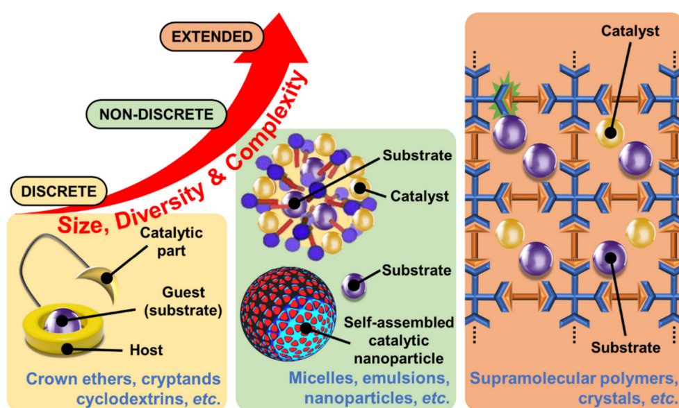
Figure 1. Some strategies for the engineering of catalytic systems from molecular building blocks by using supramolecular chemistry and self-organization.
