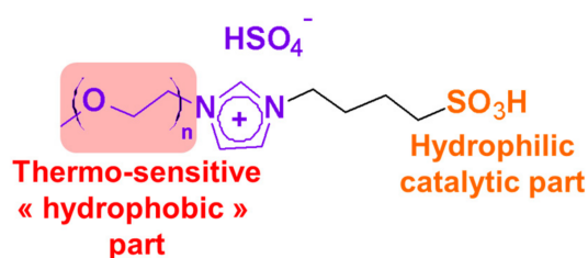
Figure 27. Thermosensitive amphiphilic Brønsted acid imidazolium salts used for the synthesis of biodiesel.
