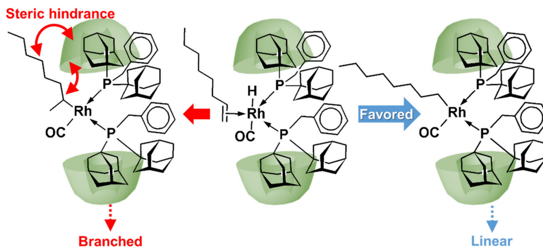
Figure 14. Supramolecular CD-based phosphorus as a first- and second-sphere ligand of rhodium.
