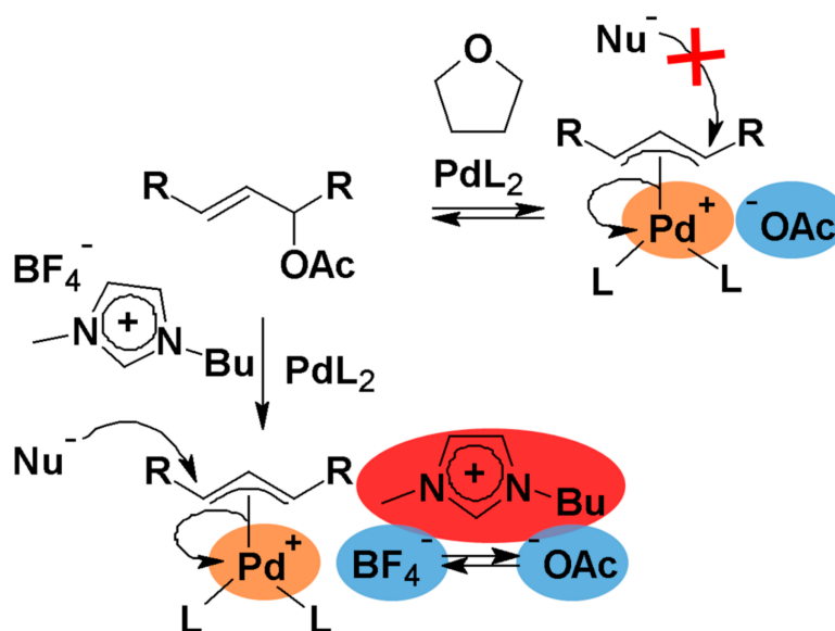
Figure 42. Effects of solvents (THF and 1-butyl-3-methylimidazolium tetrafluoroborate) on the intermediate allylpalladium (PdL 2 = active catalyst, L = phosphine, Nu − = soft nucleophile).
