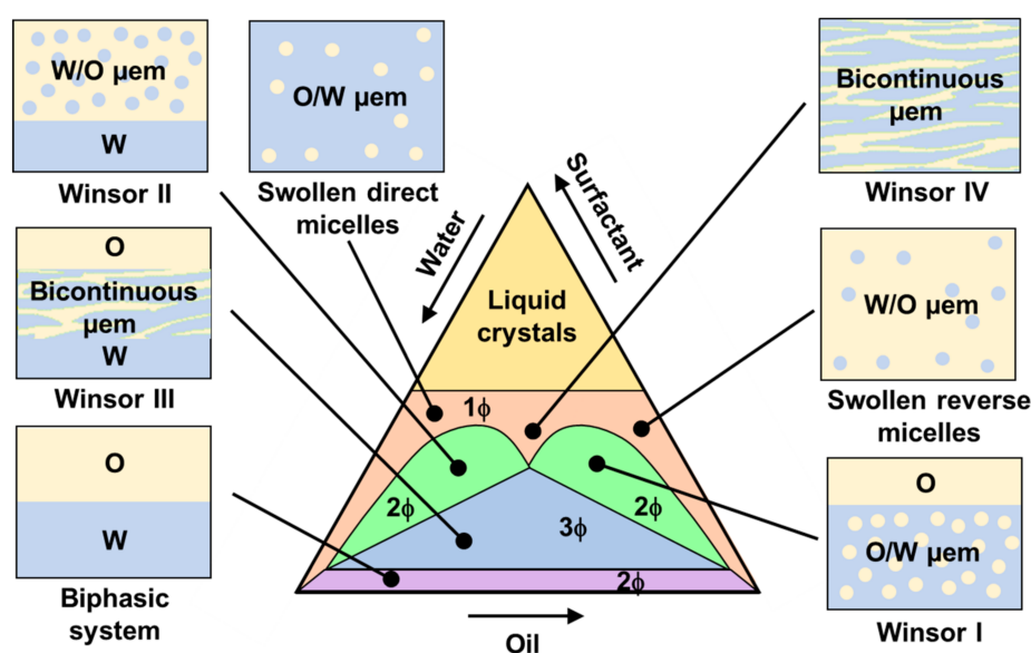
Figure 29. A schematic phase diagram of a surfactant/water/oil ternary system and microemulsion Winsor types. Note that the boundaries are arbitrary and depend on the system chosen.
