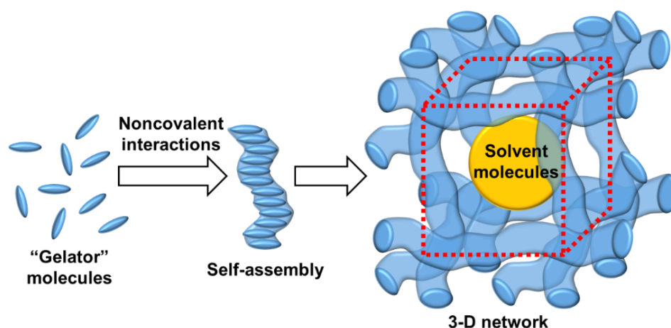
Figure 44. The formation of supramolecular gels.
