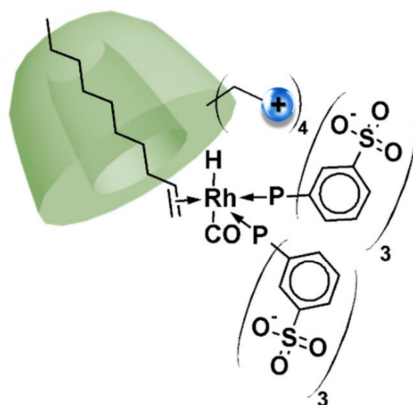
Figure 13. Rhodium complexes noncovalently bound to cationic \alpha -CD bearing 2-hydroxy-3-trimethylammoniopropyl groups to perform biphasic hydroformylation of higher olefins.
