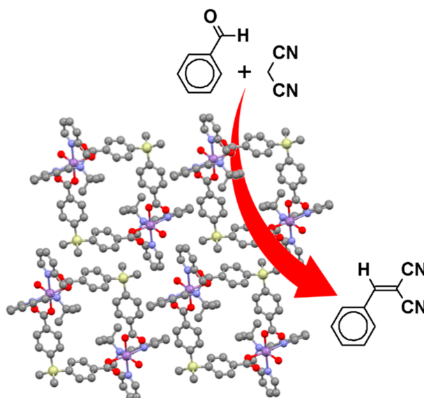
Figure 53. Catalytic Knoevenagel condensation between malononitrile and benzaldehyde catalyzed by discrete [2+2+2] molecular squares in a water environment (see CCDC reference number 1,835,561).
