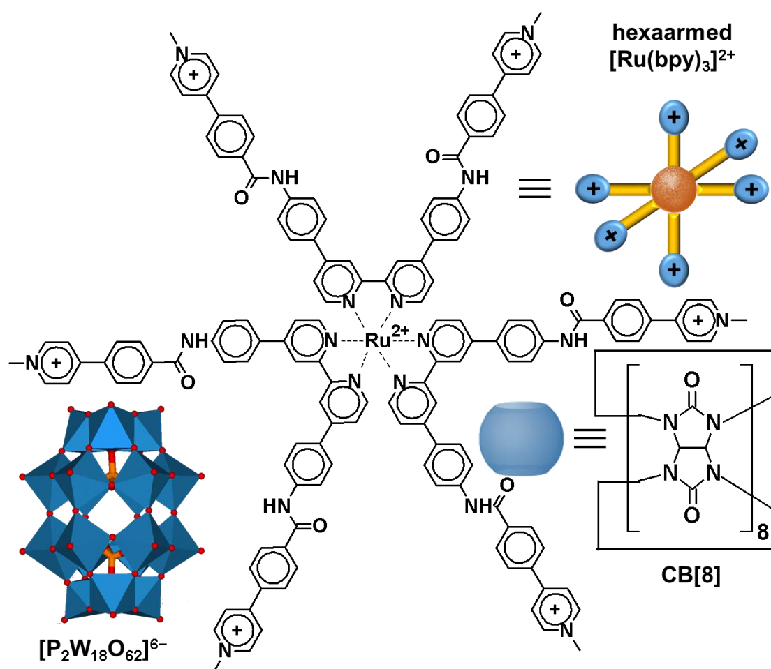
Figure 51. The structure of hexaarmed [Ru(bpy) 3 ] 2+ , CB[8], and a redox-active [P 2 W 18 O 62 ] 6- unit.
