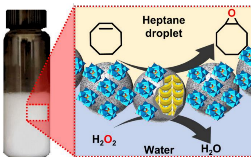
Figure 61. A schematic representation of cyclooctene epoxidation in a heptane-in-water Pickering emulsion stabilized with an amphiphilic hybrid core-shell CD/oil@ \text{PW}_{12}\text{O}_{40} NP catalyst.
