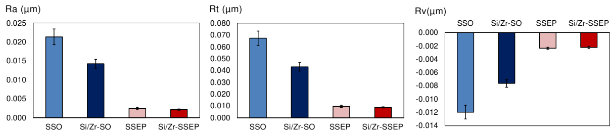
Fig. 2 Morphology multi-scale analysis results, showing roughness parameters R_a , R_t and R_v comparing coated and uncoated surfaces. The scale of pertinency [17] was approximately 2\ \mu\text{m} for these parameters.
