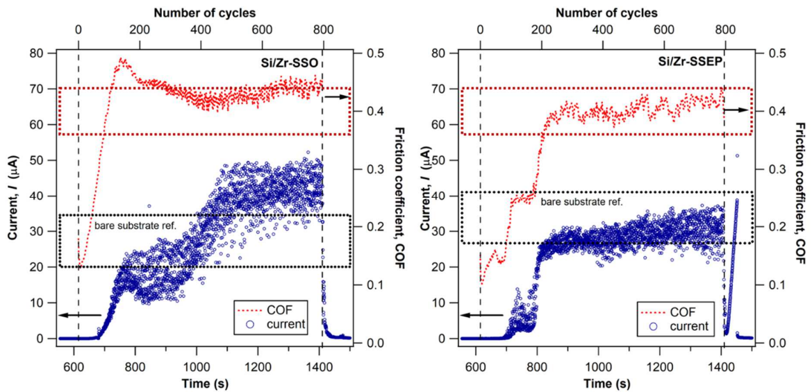
Fig. 3 Current and friction coefficient as a function of time (number of cycles). The regions delimited by the dotted lines correspond to the ranges of current and COF values for the bare substrates under similar testing conditions [14].
