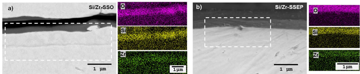
Fig. 1 SEM-EDS analysis of the cross-sections of (a) Si/Zr-SSO and (b) Si/Zr-SSEP systems.
