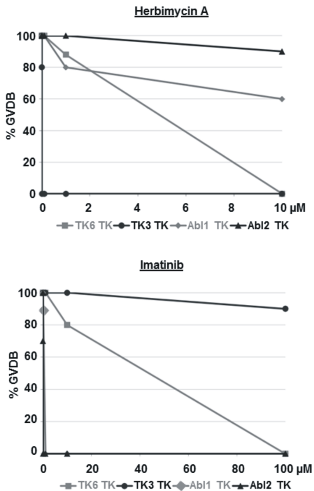
Figure 3. GVBD assays confirming SmAbl2 inhibition by Imatinib. Results of the GVBD assays performed in Xenopus oocytes to analyze schistosome-kinase activities under inhibitor influence. Herbimycin A completely inhibited SmTK3 TK enzymatic activity (circles, black) even at 0.01 μM, whereas 10 μM was needed to stop inhibit SmTK6 (squares, grey)-induced GVBD [38]. At this concentration the GVDB-inducing TK activities of SmAbl1 (rhombus, grey) and SmAbl2 (triangle, black) were reduced by only 40% or 10%, respectively. Imatinib completely inhibited GVBD induced by the TK activities of SmAbl1 (at 1 μM) or SmAbl2 (at 0.1 μM), whereas SmTK6-induced GVBD was stopped at 100 μM, a concentration that reduced SmTK3 TK-induced GVBD by only 10% [38]. doi:10.1371/journal.pntd.0002923.g003
