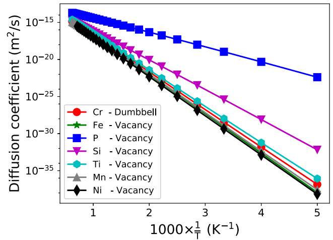
FIG. 8. Diffusion coefficients by the preferred diffusion mechanism for the various species. Calculations were performed while assuming a constant vacancy to solvent fraction of 10^{-6} .
