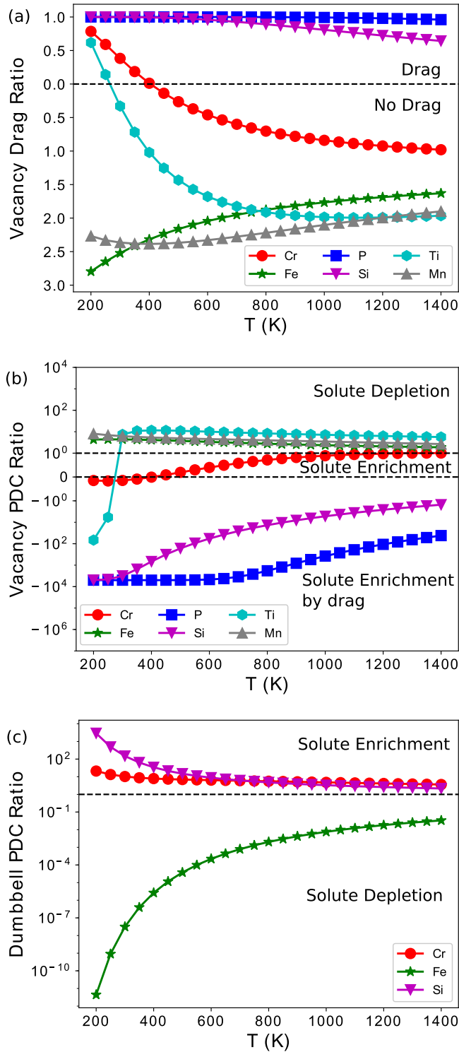
FIG. 9. (a) Vacancy drag ratio, G_V = L_{VB}^{(VB)} / L_{BB}^{(VB)} , (b) vacancy partial diffusion coefficient ratios, and (c) dumbbell partial diffusion coefficient ratios as functions of temperature. As interstitial diffusion is considered negligible for Ti and Mn, and the octahedral kickout mechanism dominates over the dumbbell mechanism for P, the three are omitted in (c).
