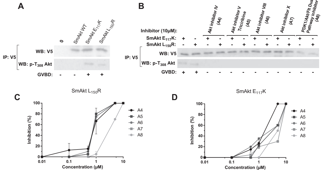
Fig. 3. Inhibition of constitutively active mutants of SmAkt expressed in Xenopus oocytes by Akt inhibitors. (A) Western blot analysis of wild type, E 117 K and L 150 R V5-tagged SmAkt proteins expressed in Xenopus oocytes. Anti V5-immunoprecipitates were analyzed in Western blot with anti-V5 or with anti-pT 308 active Akt antibodies. SmAkt E 117 K and L 150 R active kinases are recognized by anti-pT 308 serum and are able to trigger meiosis resumption in oocytes (monitored by GVBD). (B) Oocytes expressing SmAkt E 117 K or SmAkt L 150 R were incubated with 10 μM of each Akt inhibitor (A4–8). Anti V5-immunoprecipitates were analyzed as in (A). The five compounds inhibit phosphorylation and activity of SmAkt mutants. (C, D) Oocytes expressing SmAkt L 150 R (C) or E 117 K (D) were incubated with variable concentrations of Akt inhibitors (A4–8). For each condition, percentages of oocytes with GVBD were calculated and the results expressed in % of inhibition of maturation using as reference oocytes without inhibitor (mean ± SEM of three independent experiments).
