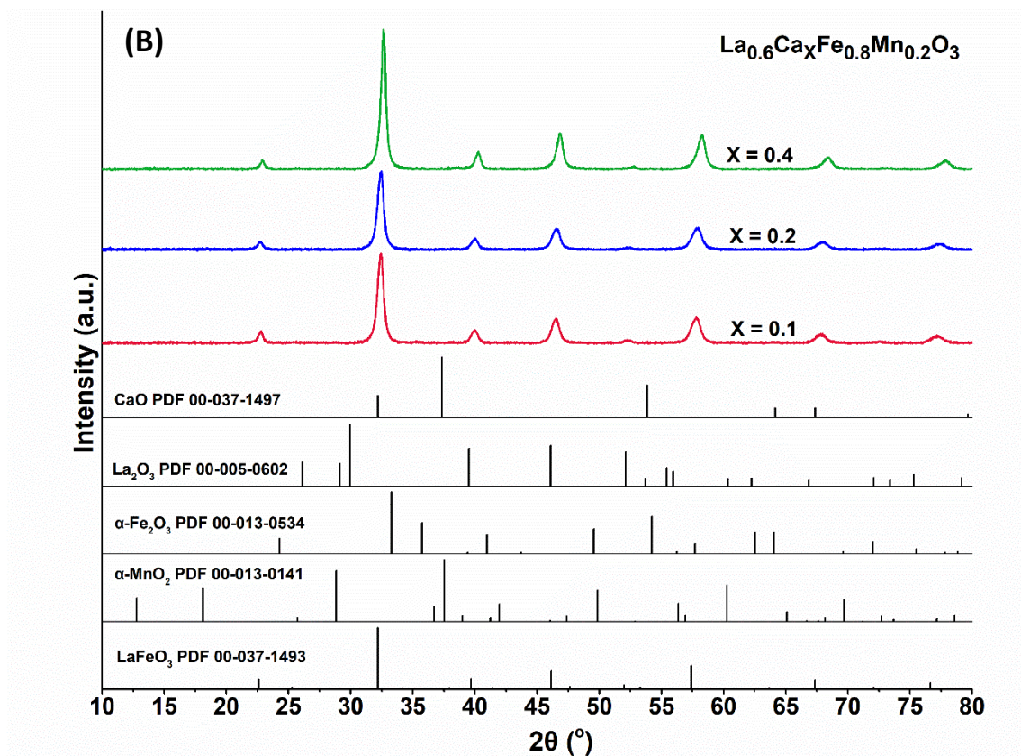
Fig. 1. XRD diffractograms of \text{LaFeO}_3 , La-deficient \text{La}_{0.7}\text{Fe}_{1-y}\text{Mn}_y\text{O}_3 perovskites with y = 0 or 0.2 (A), and dual substituted \text{La}_{0.6}\text{Ca}_x\text{Fe}_{0.8}\text{Mn}_{0.2}\text{O}_3 perovskites with x = 0.1, 0.2 or 0.4 (B).
