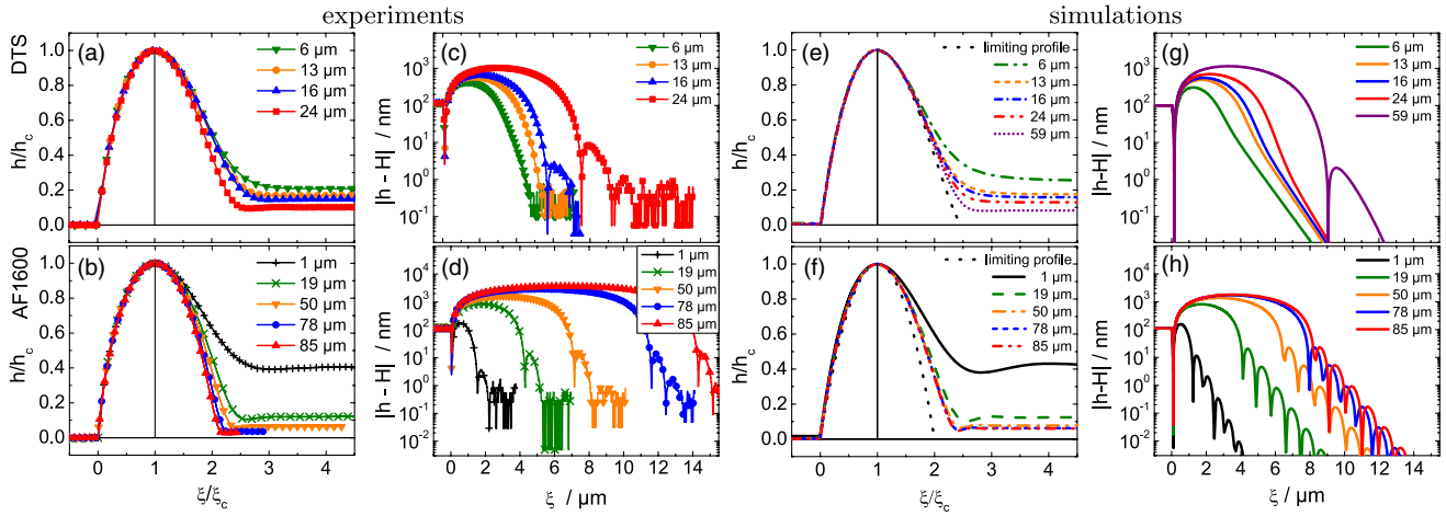
FIG. 2 (color online). (a)—(d) AFM scans of rim profiles of straight fronts of a thin film (PS(10.3 kg/mol), H = 115(5) nm) on DTS [(a),(c)] at 110 °C and AF1600 [(b),(d)] at 120 °C, recorded at various travelled distances D as noted in the legend. (e)—(h) Snapshots of the unperturbed numerical simulations taken at the travelled distance D given by the experiments in (a)—(d). Normalized h , \xi with the coordinates at maximum h_c , \xi_c illustrate the approach to an asymptotic profile. The vertical straight line helps to visualize the asymmetry between the front and rear of the ridge. On DTS, the semilogarithmic representation of |h - H| indicates the transition from a monotonically decaying tail to an oscillatory decay. In the presence of slip, both experiments on DTS and numerical calculations of the strong-slip model show a morphological transition of the rim profile [45]. On AF1600, oscillatory profiles are present right from the early stage ( D = 1 \mu\text{m} ) of the dewetting process [46].
