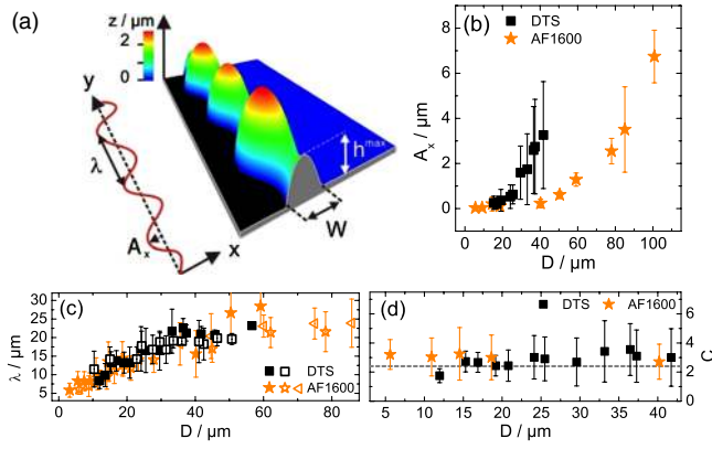
FIG. 3 (color online). (a) AFM image of an undulated rim (10.3 kg/mol at 125°C on AF1600, D = 97 \mu\text{m} , t = 6360 \text{ s} , scan size: 15 \mu\text{m} \times 90 \mu\text{m} ) with parameters characterizing the undulation: rim width W , rim height h^{\max} , wavelength \lambda , and lateral amplitude A_x . (b) Lateral amplitude A_x of the rim instability in regime I and II determined from AFM images of a PS film (10.3 kg/mol, H = 115(5) \text{ nm} , 120°C) show distinct differences on DTS and AF1600. (c) For the studied film thicknesses H = 110\text{--}130 \text{ nm} and molecular weights (10.3 and 13.7 kg/mol), represented by different symbols, the wavelength \lambda of the instability grows continuously with dewetted distance D and does not depend on the substrate. (d) The Rayleigh ratio C = \lambda/W (where W was precisely determined from AFM images, filled symbols) as a function of D for both, DTS and AF1600 shows a good agreement between experiments and theory (dashed line) [13].
