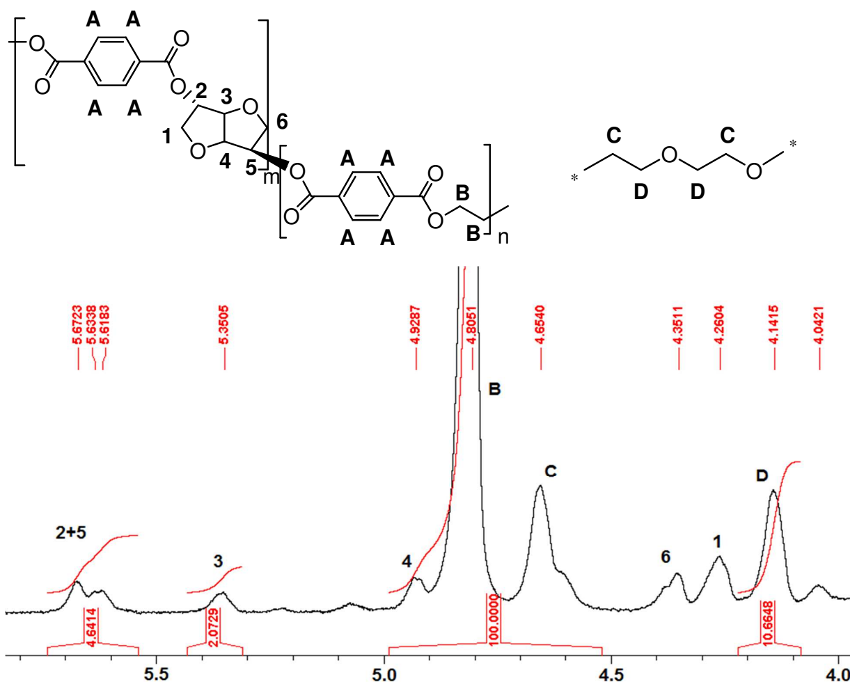
Figure 1. 1 H NMR spectra of a typical PEIT (entry 2) at 300 MHz in a mixture of deuterated chloroform and deuterated trifluoroacetic acid (3:1 vol%) in the 4-6 ppm zone and assignments.
