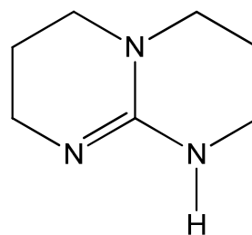
1,5,7-triazabicyclo[4.4.0]dec-5-ene (TBD)
