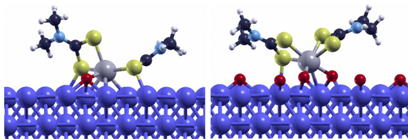
Figure 8. Optimized configuration for mMoDTC adsorbed on the clean (left) and oxygen-passivated (right) iron (110) surfaces.
