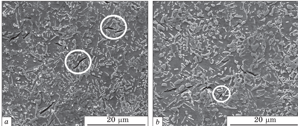
Fig. 7. SEM surface observation of the external surface of the sample fatigued at \Delta\epsilon_t = 1.4\% after etching
