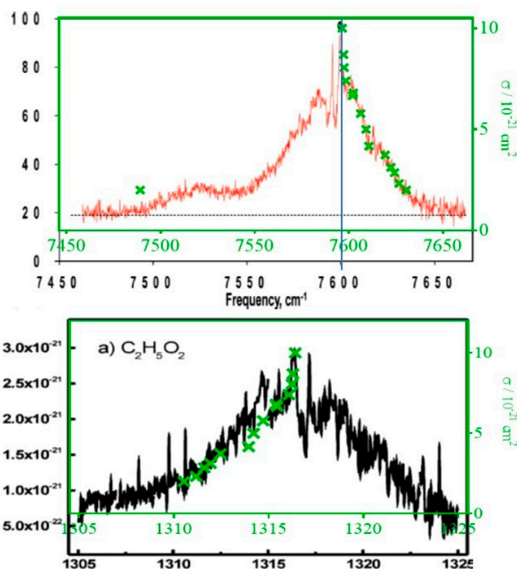
Figure 7. C_2H_5O_2 absorption coefficients at different wavelengths obtained in this work (green crosses and green axis), overlaid onto the spectrum obtained by Melnik et al. [17], Reprinted with permission from [17], Copyright 2010 American Chemical Society) and Atkinson and Spillman [11] (lower graph, Reprinted with permission from [11], Copyright 2002 American Chemical Society). In the upper graph the data have been shifted by 4 cm^{-1} , and in both graphs our data have been scaled on the y -axis, i.e., apparently there is a baseline shift in both comparisons.
