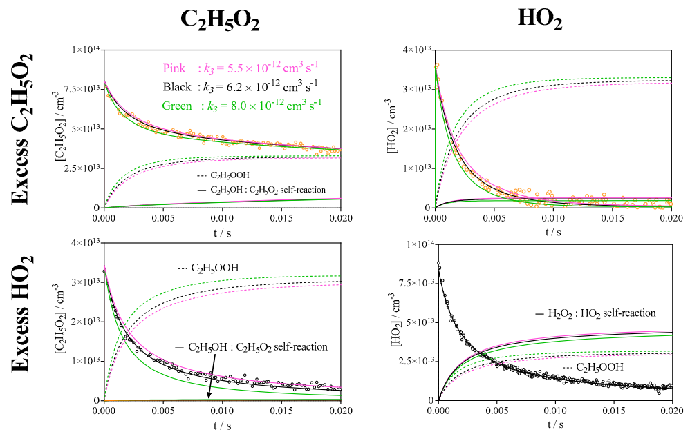
Figure 5. Experimental profiles taken under excess C_2H_5O_2 conditions (upper graphs) and under excess HO_2 conditions (lower graph). The dashed lines represent modelled profiles of C_2H_5OOH , the product from (R3), while the full lines represent the product of the corresponding self-reaction ( C_2H_5OH for C_2H_5O_2 and H_2O_2 for HO_2 ). Different colours represent the result from a model with different k_3 .
