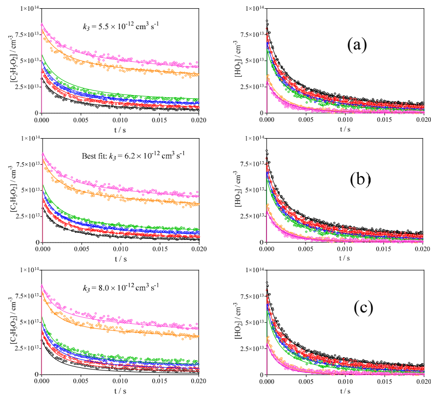
Figure 6. C_2H_5O_2 (left graphs) and HO_2 (right graphs) concentration time profiles for a total radical concentration of 1.2 \times 10^{14} \text{ cm}^{-3} . C_2H_5O_2 absorption time profiles have been converted using \sigma = 1.0 \times 10^{-20} \text{ cm}^2 . Centre graphs (b): best fit with k_3 = 6.2 \times 10^{-12} \text{ cm}^3 \text{ molecule}^{-1} \text{ s}^{-1} , upper graphs (a): model with of k_3 = 5.5 \times 10^{-12} \text{ cm}^3 \text{ molecule}^{-1} \text{ s}^{-1} , lower graphs (c): model with k_3 = 8.0 \times 10^{-12} \text{ cm}^3 \text{ molecule}^{-1} \text{ s}^{-1} .
