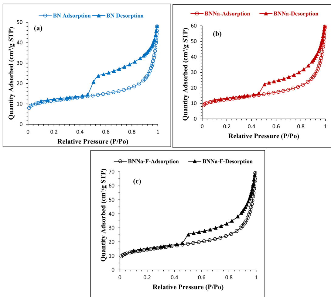
Figure 8. N_2 adsorption-desorption isotherms of (a) BN; (b) BNNa; (c) BNNa-F. BN: raw sample; BNNa: Na-Homoionic coarse fraction of 40 \mu m ; BNNa-F: Na-Homoionic form of the Fine fraction ( <2 \mu m ).
