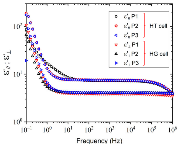
Figure S1. Relative permittivity of three purified LC mixtures as a function of frequency. Measurements were taken at 1 V and room temperature (20 °C) using 20 \mu\text{m} cells in homogeneous and homeotropic alignments. P stands for purified LC mixtures.
