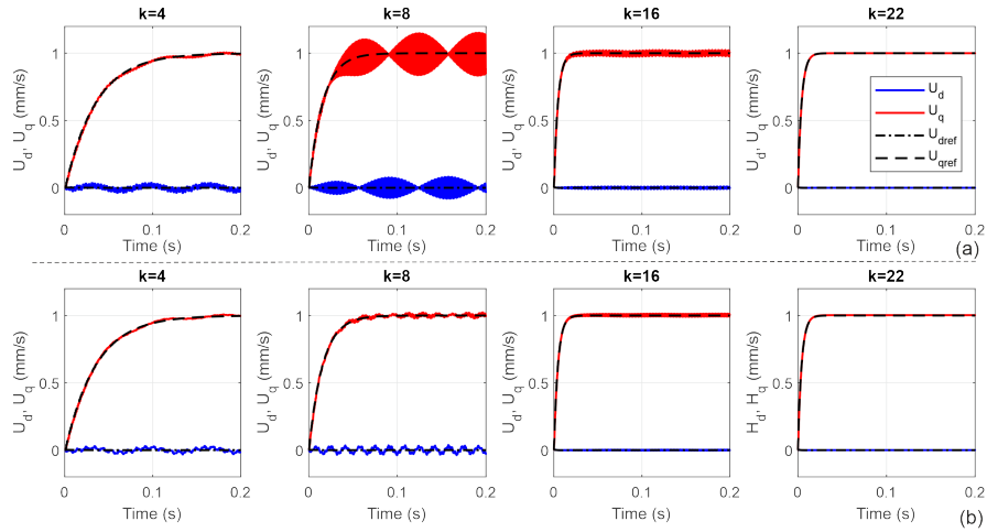
Figure 16: Obtained simulation responses with the classical (a) and the proposed (b) method for calculating the modal filter weighting gains, U_{dref} and U_{qref} correspond the ideal modal responses
