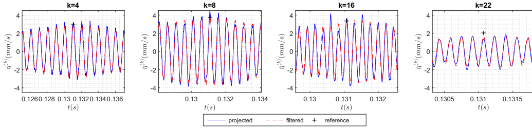
Figure 21: Extracted modal velocities \dot{\eta}^{(k)} of the controlled modes in absence of external perturbation, the modal velocities reference at the focusing time \dot{\eta}_f^{*(k)} are represented by the symbol +.
