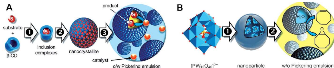
A. Principle of CD/substrate combination to perform interfacial catalysis in a O/W emulsion with a catalyst in aqueous phase (PAC). B. Principle of epoxidation in a W/O emulsion stabilized by catalytic nanoparticles formed by a POM and alkylammonium cations (PIC). 3
