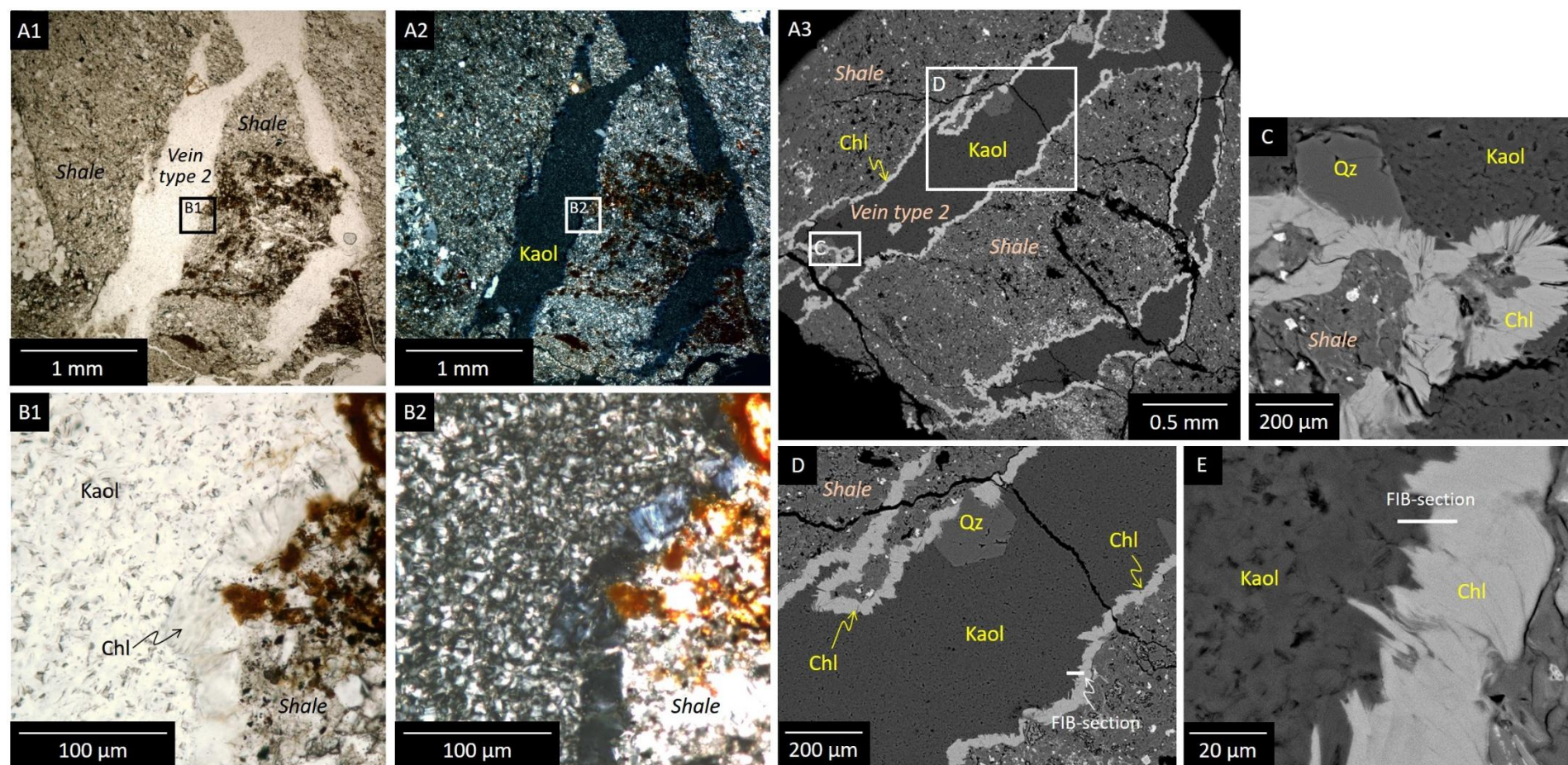
1 2 Figure 4: Optical microscope and SEM images of a carboniferous shale sample. (A) and (B): images of the large view of the veins/shale contact by plain light microscopy (A1 and B1), 3 crossed-polarized light microscopy (A2 and B2) and SEM (backscattered-electrons) (A3), showing kaolinite vein (type 2) running through the shale. A: images highlight the wide 4 expanse of the chlorite fringe along the kaolinite/shale interface. All kaolinite areas are surrounded by chlorite. (C) and (D) images are located. (B): plain light (B1) and 5 crossed-polarized light (B2) microscopy images of the vein/shale contact, highlighting the chlorite fringe at the kaolinite/shale interface. (C): hairy chlorite seems to grow from the 6 shale to kaolinite. (D): chlorite fringe on either side of a kaolinite vein. FIB section is located. (E): zoom of (D) image detailing the kaolinite/chlorite contact. Qz: quartz; Kaol: kaolinite; 7 Chl: chlorite.
