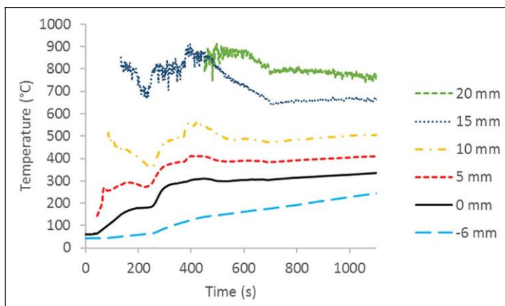
Figure 4. Temperature as a function of time at different heights in 6-mm-thick sample and in char of PP with 10 wt% EG during cone calorimeter experiment (external heat flux = 35 \text{ kW/m}^2 )—0 mm is the height of the surface exposed to heat flux. Measurements are made in the center of the plate.
