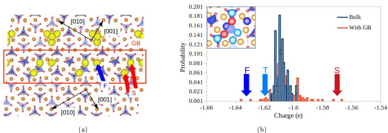
Figure 8: Results of Bader analysis performed on the non-stoichiometric E2 GB complex (see Fig.7b). Figure (8a) : isosurfaces of charge density (level at 0.05e) belonging to different O ions. Figure (8b) : O charge distributions in a perfect crystal environment (blue) and in the system containing the GB (orange), the red arrow points the O ions highlighted in red in the sketch zooming on the interface, the blue arrow points the O ions highlighted in dark blue in the sketch and the blue circle points the O ions highlighted in light blue in the sketch.
