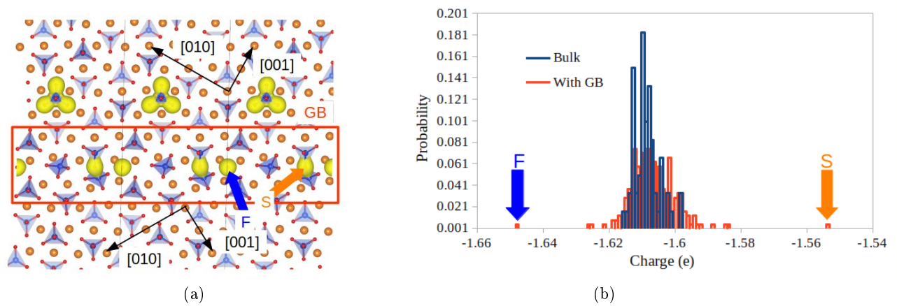
Figure 5: Results of Bader analysis performed on the E2 stoichiometric GB complexion (see Fig.4b). Figure (5a) : isosurfaces of charge density (level at 0.05e) belonging to different O ions, figure (5b) : O charge distributions in a perfect crystal environment (blue) and in the system containing the GB (orange).
