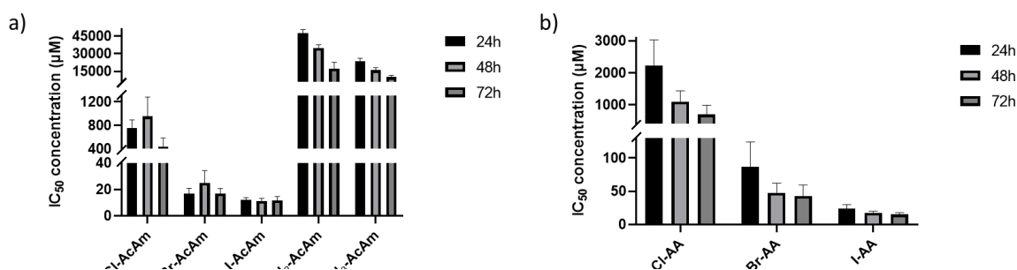
Figure 1.2.: IC_{50} values ( \mu M) determined after 24h, 48h and 72h for, (a) chloro- (Cl-AcAm), bromo- (Br-AcAm), iodo- (I-AcAm), dichloro- (Cl 2 -AcAm), trichloroacetamide (Cl 3 -AcAm) and, (b) chloro- (Cl-AA), bromo- (Br-AA) and iodoacetic acid (I-AA). Error bars represent the 95% confidence interval.
