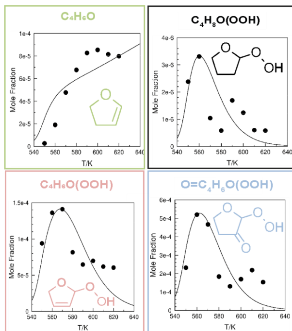
Fig. 55. Profiles of selected species during THF oxidation in a JSR ( \phi=0.5 , 0.5% THF, 10 bar, residence time of 2 s): experimental signal profiles (dots) [590] scaled to the maximum computed mole fraction using the model of Fenard et al. [283]. (lines). Reproduced from Ref. [590] with permission of American Chemical Society.
