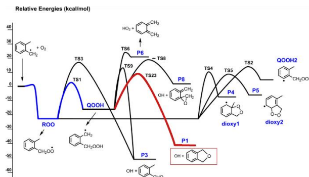
Fig. 36. Relative energies of major reaction pathways on PES of o -xylyl + O 2 at 0 K in kcal/mol (the initial bimolecular reactants are set to energy zero)—reproduced from Ye et al. [543] with permission of Elsevier.
