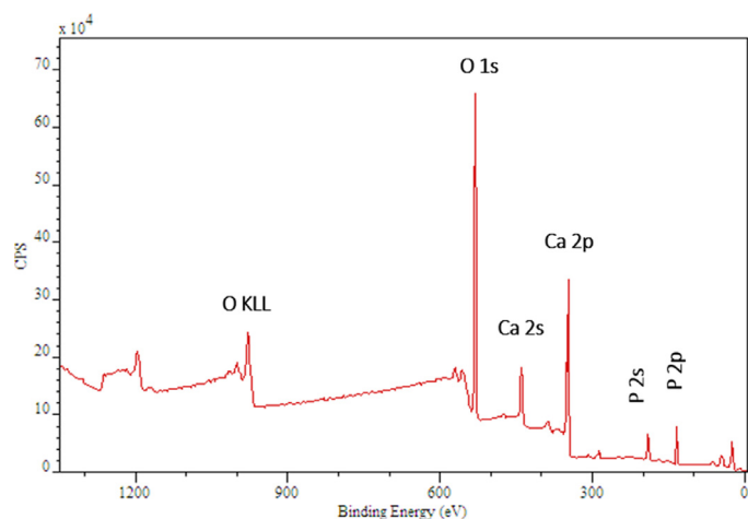
Fig. 8. XPS survey spectrum measured of nHAp.
