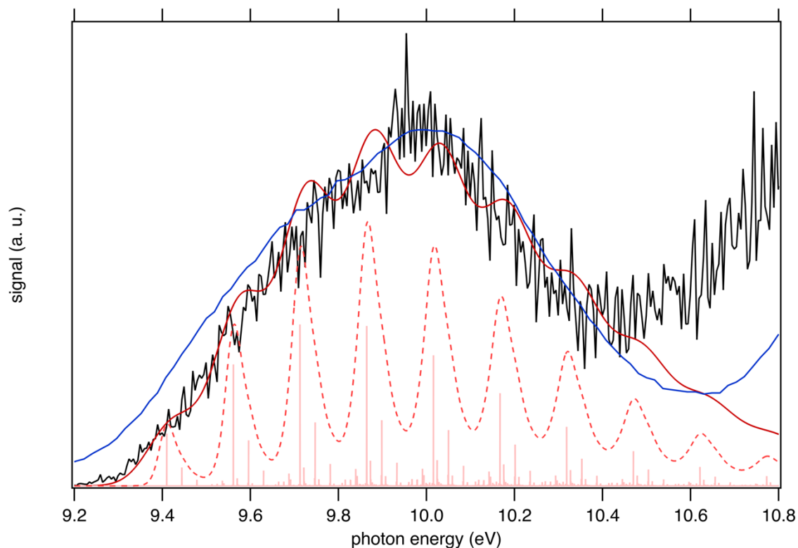
FIGURE 8. Sum of the SPES of m/z 57 and 90 (black line) compared to a reference PES of tBuOOH (blue line) from Nagaoka et al. [59] and two simulated spectra of tBuOOH using the current FC simulation. The simulations are based on the computed stick spectrum (light red sticks) convoluted with 20 meV (dashed red line) and 60 meV (dark red line) HWHM Gaussians. The latter corresponds to the spectrum in FIGURE 7 in which modes 42, 41, 40, and 37 have been removed. The simulations have been shifted by 156 meV from the calculated AIE by CC calculations.
