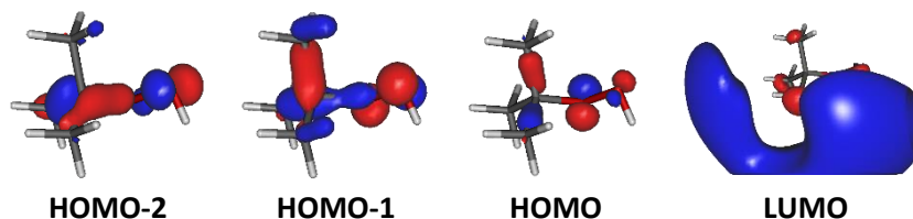
FIGURE 6. Outermost molecular orbitals of tBuOOH as computed at the HF/aug-cc-pVTZ level.
