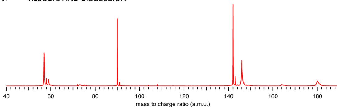
FIGURE 1. Mass spectrum recorded by synchrotron photoionization of a tBuOOH/ n -decane mixture in helium integrated over the 9.0 – 11.0 eV photon energy range.
