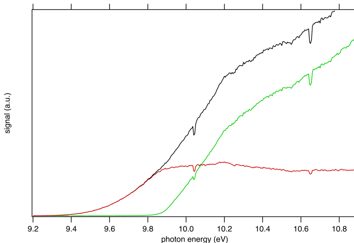
FIGURE 2. PEPICO spectra of the tBuOOH parent ion m/z 90 (red line) and its fragment m/z 57 (green line) formed by dissociative ionization energy in the 9.2 – 10.8 eV energy range. The black curve is the sum PEPICO spectra of m/z 57 and 90. Note that for the sake of clarity the uncertainties, which are small, are not represented on this graph. The dips at 10.033 eV and 10.644 eV originate from absorption in the gas filter (see experimental methods above) and correspond to the 5s and 5s' Kr absorption lines.
