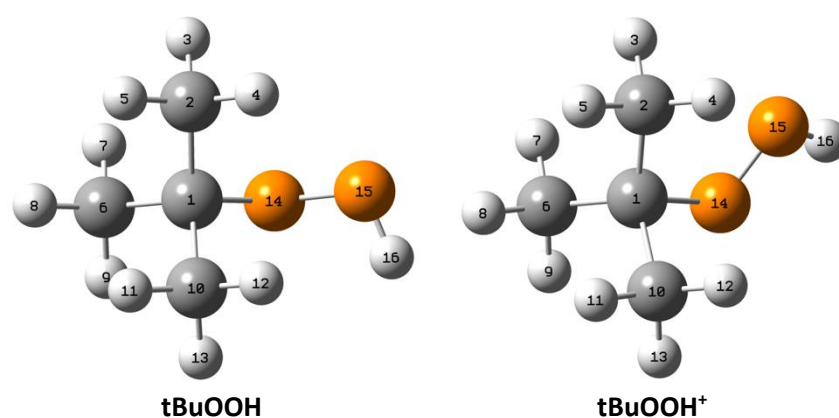
FIGURE 5. Optimized equilibrium structures of neutral tBuOOH and of its cation in their electronic ground states as optimized at the PBE0/aug-cc-pVTZ level. The numbering of the atoms used presently is also given.
