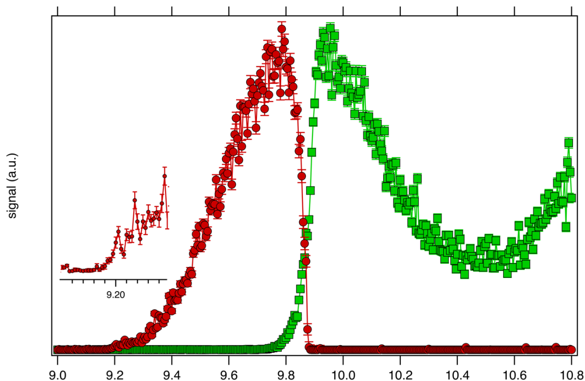
FIGURE 3. SPES of m/z 57 (green squares) and 90 (red dots) recorded by synchrotron photoionization of a tBuOOH/ n -decane mixture in helium. The inset shows a blown-up view around the ionization onset.
