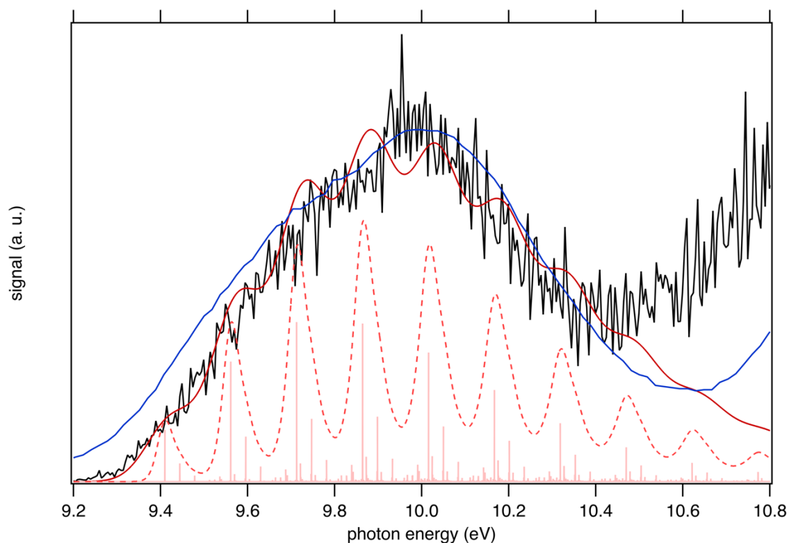
FIGURE 8. Sum of the SPES of m/z 57 and 90 (black line) compared to a reference PES of tBuOOH (blue line) from Nagaoka et al. [59] and two simulated spectra of tBuOOH using the current FC simulation. The simulations are based on the computed stick spectrum (light red sticks) convoluted with 20 meV (dashed red line) and 60 meV (dark red line) HWHM Gaussians. The latter corresponds to the spectrum in FIGURE 7 in which modes 42, 41, 40, and 37 have been removed. The simulations have been shifted by 156 meV from the calculated AIE by CC calculations.
