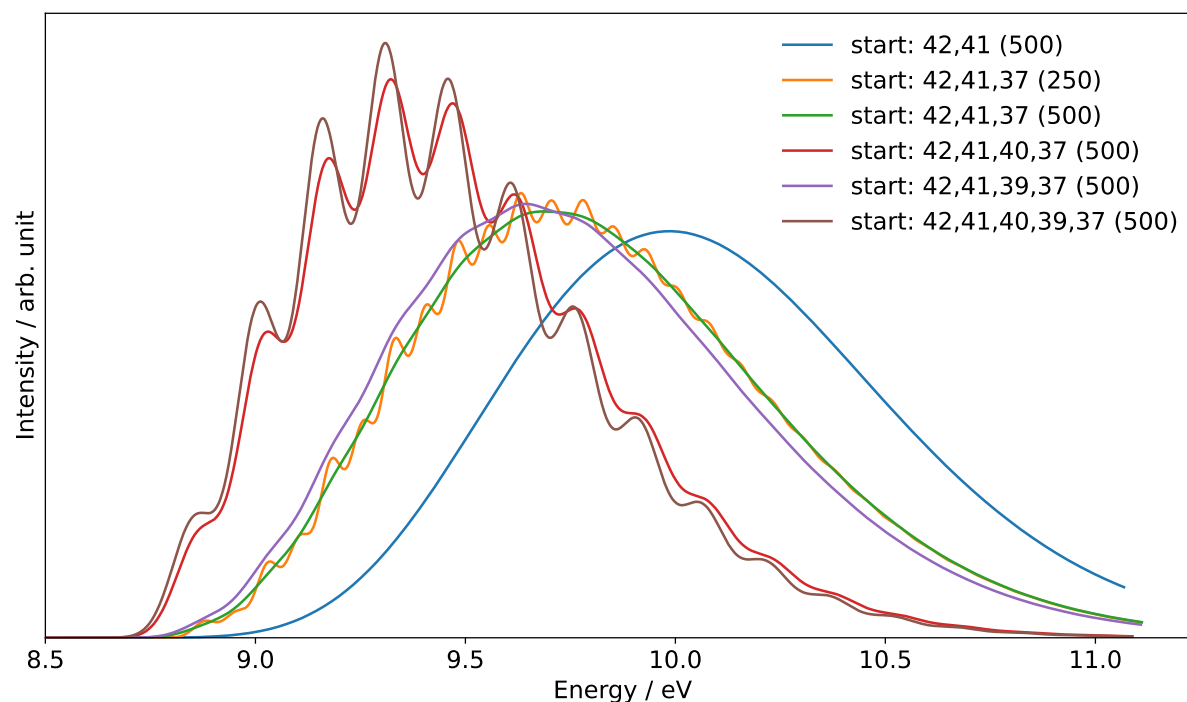
FIGURE 7: Reduced-dimensional PES spectrum at the FC level using the time-dependent (TD) formalism, choosing different sets of normal modes to exclude in the initial state at the beginning of the calculations. The selected modes are listed in the legend (“start”). Gaussian distribution functions were used to reproduce the experimental broadening. The half width at half maximum (HWHM), given in \text{cm}^{-1} , is indicated between parentheses.
