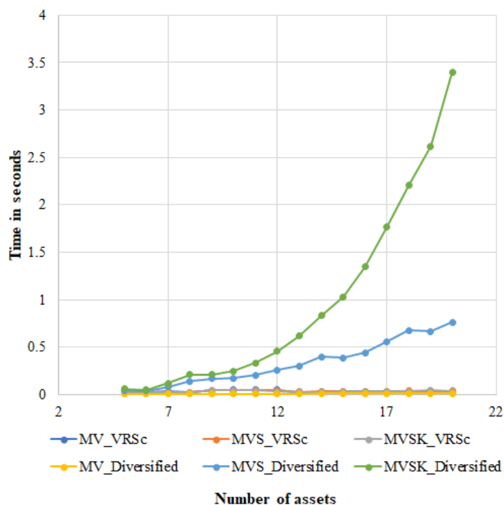
Figure A.1: Average CPU time for optimizing one observation
