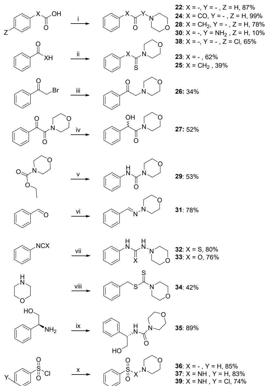
Scheme 2. Synthetic pathway of compounds 22–39 a . a Reagents and conditions: (i) COCl 2 , DIPEA, appropriated amine, CH 2 Cl 2 , r.t., 10%–99%; (ii) S 8 , morpholine, DMF, 39%–62%; (iii) morpholine, K 2 CO 3 , MeCN, r.t., 34%; (iv) NaBH 4 , MeOH, r.t., 52%; (v) (1) POCl 3 , MeCN, 50 °C, (2) aniline, DIPEA, 0 °C to r.t., 53%; (vi) 4-amino-morpholine, MgSO 4 , CH 2 Cl 2 , r.t., 78%; (vii) 4-amino-morpholine, CH 2 Cl 2 , r.t., 76%–80%; (viii) (1) CS 2 , Et 2 O, r.t., (2) (thiocyanatomethyl)benzene, ACN, r.t., 42%; (ix) morpholine-4-carbonyl chloride, DIPEA, CH 2 Cl 2 , r.t., 89%. (x) Appropriated amine, Et 3 N, r.t., 83%–85%.
