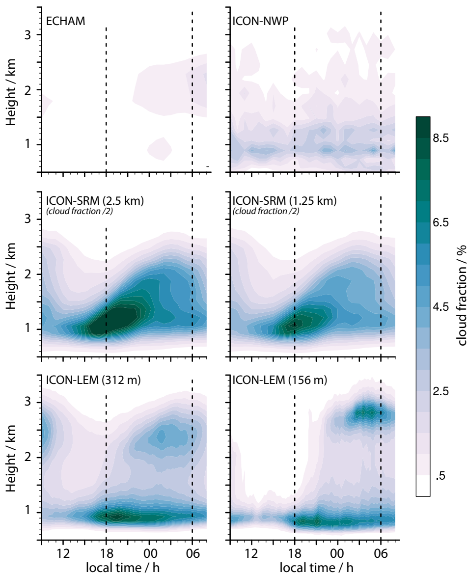
Fig. 21. Composite diel cycle of cloudiness over the BB domain (43°W to 60°W, 12°N to 16.5°N). Differences between the 312 m and 156 m meshes are largely due to the fact that a smaller domain (not shown) is used for the finer mesh. Dashed lines demarcate sunset and sunrise. Note that ICON-SRM cloud fractions are twice the indicated value.
