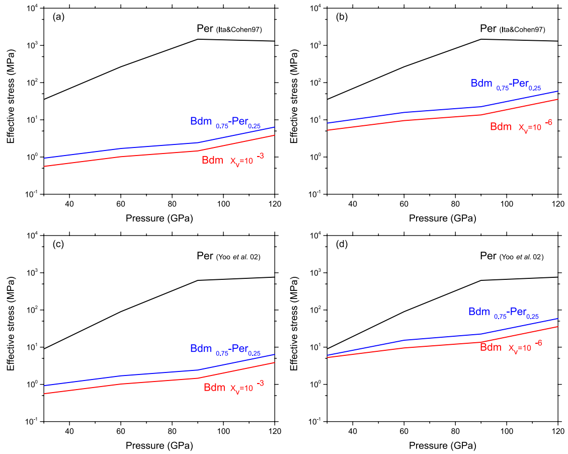
Extended Data Fig. 5 | Pressure dependence of the aggregate rheology. The flow stress \bar{\sigma}_0 (blue line) for a bridgmanite (Bdm) – periclase (Per) aggregate (volume fraction of MgO: 0.25), is obtained with the POSO Self-Consistent scheme, for vacancy concentrations of 10 -3 and 10 -6 in bridgmanite and two
