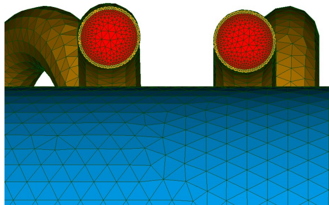
Figure 5. Considered mesh.
