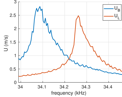
Figure 4: Frequency response of the vibration speed for each mode; U_B is the vibration speed for the bending mode and U_L is for the longitudinal mode
