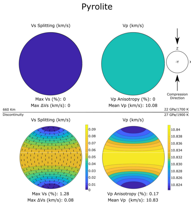
Fig. 5. Seismic velocities in pyrolite at conditions above and below the 660 km discontinuity. Both V_S splitting and V_P anisotropy are plotted in units of km/s. Black tick marks in V_S anisotropy plots indicate the fast shear wave polarization direction. Plots are oriented so that compression is in the vertical direction. Details on their calculations and numerical values of the corresponding densities and elastic moduli are provided in the Supplementary Materials.
