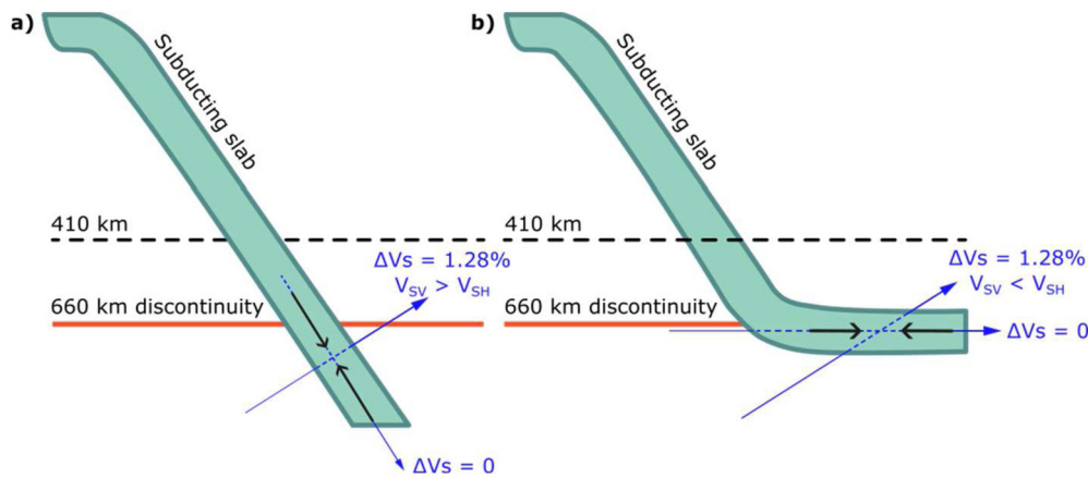
Fig. 6. Scenarios for anisotropy in a subducting slab below the ‘660’. Blue arrows denote shear wave propagation directions with corresponding splitting values. Black arrows indicate compression direction. a) Subducting slab impinging on the more viscous upper-lower mantle below 660 km depth. b) Subducting slab bending along the 660 km discontinuity creating a horizontal compressive stress.
