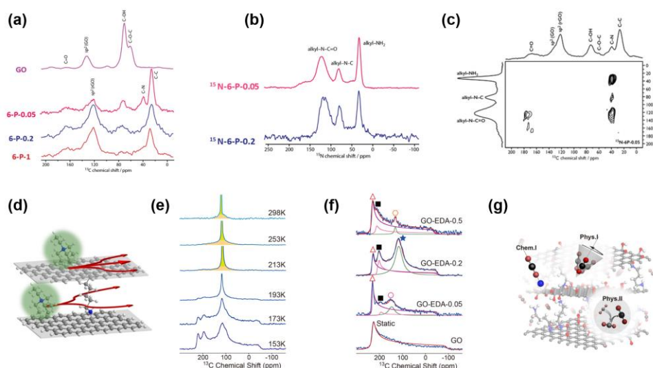
Figure 10. (a) ^1\text{H}\rightarrow^{13}\text{C} CP/MAS NMR spectra of graphene oxide (GO) and unreduced pillared materials (6-Ps) with varied diamine amount, (b) ^1\text{H}\rightarrow^{15}\text{N} CP/MAS NMR spectra of ^{15}\text{N} -labeled 6-P-0.05 and 6-P-0.2, (c) ^{13}\text{C} - ^{15}\text{N} HETCOR NMR spectrum of 6-P-0.05 and (d)
