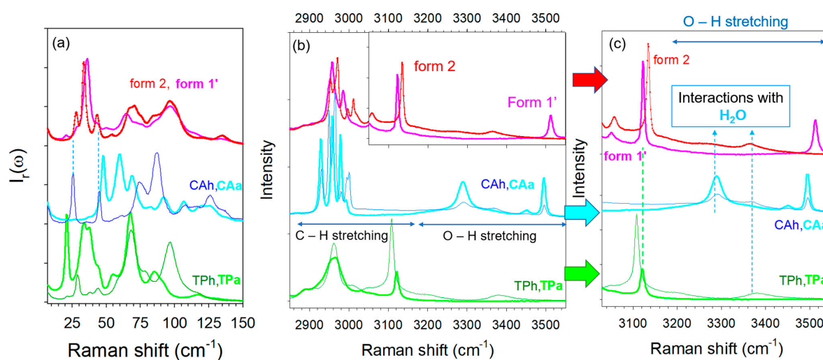
Figure 2. Raman spectra of the two pseudo polymorphic forms of co-crystals, form 1', form 2, and single components: anhydrous and hydrated theophylline (TPa, TPh), anhydrous and hydrated citric acid (CAa, CAh), (a) in the low-frequency region, (b) in the C–X stretching region (X = C, O), (c) in the O–H stretching region.
