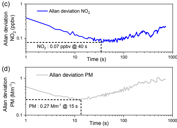
Figure 5 Time series simultaneous measurements of \text{NO}_2 concentration using BBCEAS and \text{NO}_x analyzer AC-31M (a) and PM light extinction (b) in indoor air. Allan variance plots of the \text{NO}_2 measurement (c) and PM measurement (d) showing the instrument stability induced optimal integration time of 40 s for \text{NO}_2 and 15 s for PM, respectively.
