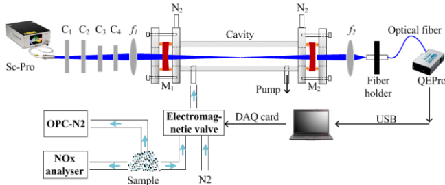
Figure 1 Schematic of the BBCEAS instrument developed in the present work. A \text{NO}_x analyzer (Environment SA, AC-31 M) and an optical particle counter (OPC-N2, Alphasense) were used for side-by-side inter-comparison measurements of \text{NO}_2 and PM. SC-Pro: supercontinuum source; M_1 , M_2 : high reflectivity mirror; QEPro: spectrometer; C_1 , C_2 : optical attenuators; C_3 , C_4 : optical filters; f_1 , f_2 : focusing lens.
