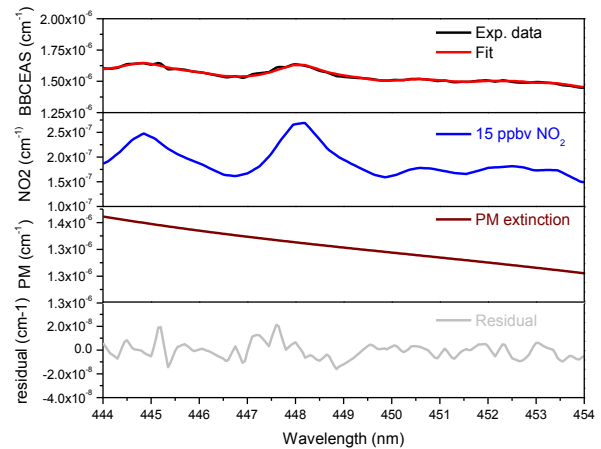
Figure 7 Typical experimental BBCEAS spectrum (black) accompanied with its fit (red), decomposed absorption spectrum of 15 ppbv \text{NO}_2 (blue) and PM extinction coefficient of 134 \text{ Mm}^{-1} . The residual (grey) between the measurement and the fit results in a standard deviation of 6.4 \times 10^{-9} \text{ cm}^{-1} .
