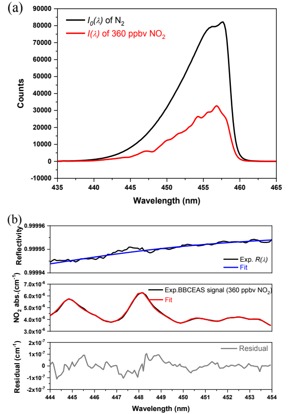
Figure 3 (a) Light intensities I_0(\lambda) and I(\lambda) leaking from the cavity without and with absorbing gas (360 ppbv NO_2 ), respectively. (b) Upper panel: Experimental mirror reflectivity (black) and its fit (blue). Middle panel: Typical experimental light absorption coefficient (black) of 360 ppbv NO_2 and its fit (red). Lower panel: Residual (grey) between the measurement and the fit, with a standard deviation of 4.0 \times 10^{-8} \text{ cm}^{-1} .
