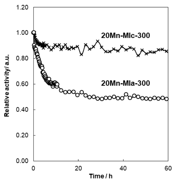
Figure 14. Evolution of the relative activity for \text{MnO}_x -SBA-15 catalysts (20 wt.% Mn) prepared by different synthesis methods at a reaction temperature of 130 °C at a R.H. of 50% at 25 °C.
