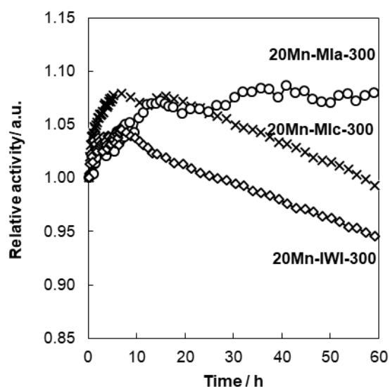
Figure 13. Evolution of the relative activity for \text{MnO}_x -SBA-15 catalysts (20 wt.% Mn) prepared by different synthesis methods at a reaction temperature of 170 °C.
