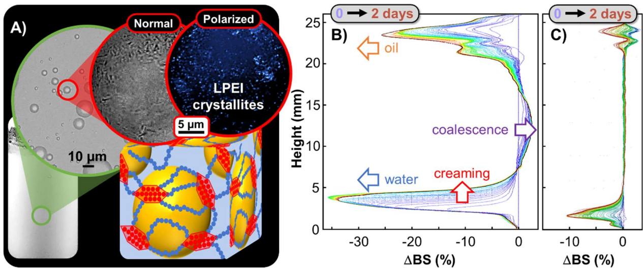
Figure 5. Macroscopic and microscopic (under normal and polarized light) views of paraffin-in-water emulsions stabilized by 0.5 wt.% LPEI with interpretation (A) and backscattering ( \Delta BS ) versus sample height and time at 25 °C for 0.5 and 2 wt.% LPEI emulsions (B and C, respectively).
